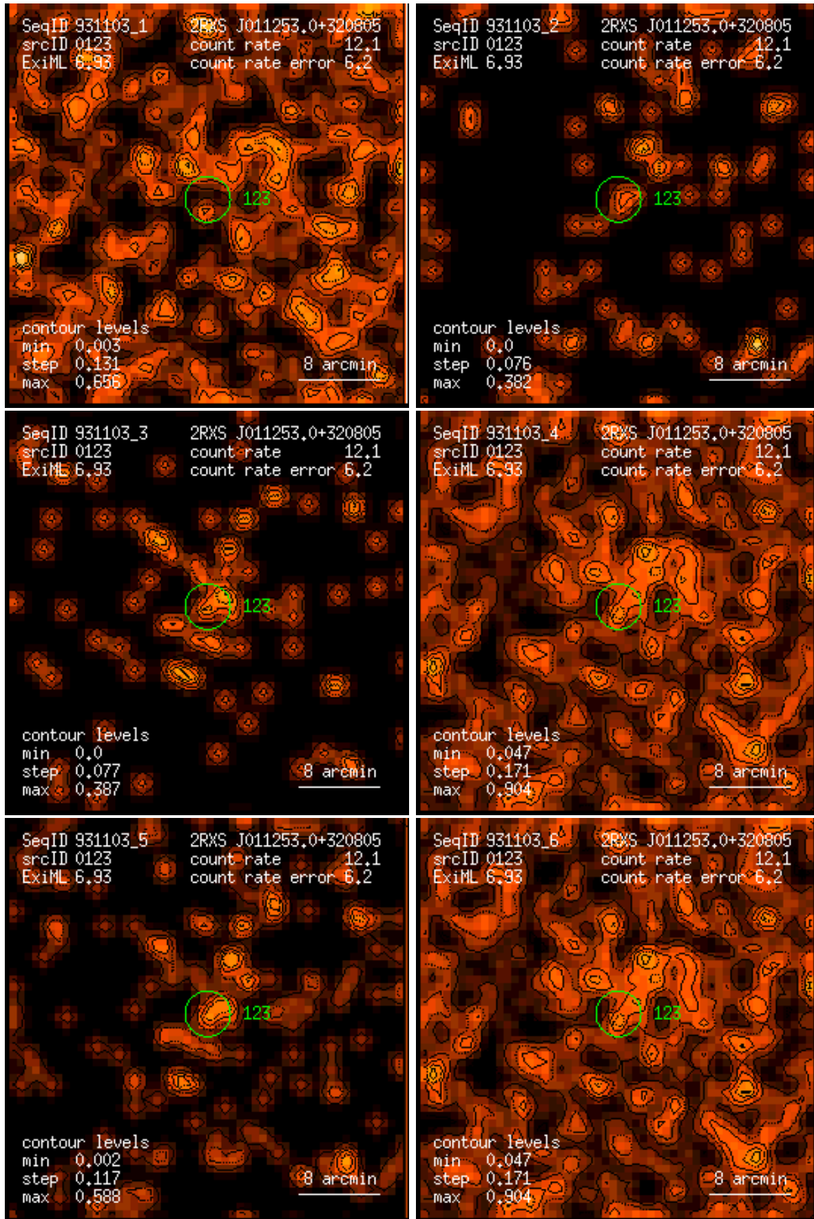
Figure 123: RASS 931103: detection 0123: band rate images, Gaussian filter: (1) PSPC channels 11 – 41, (2) 52 – 90, (3) 91 – 201, (4) 11 – 235, (5) 52 – 201, (6) 11 – 201. Broad band rates in counts/ks. Band rate contour levels in counts/ks/arcmin 2 .
