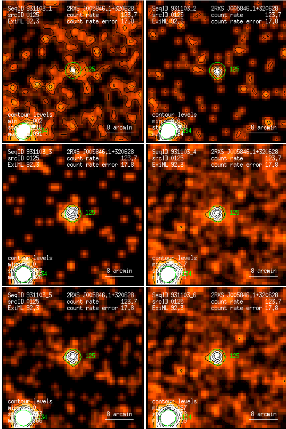
Figure 125: RASS 931103: detection 0125: band rate images, Gaussian filter: (1) PSPC channels 11 – 41, (2) 52 – 90, (3) 91 – 201, (4) 11 – 235, (5) 52 – 201, (6) 11 – 201. Broad band rates in counts/ks. Band rate contour levels in counts/ks/arcmin 2 .
