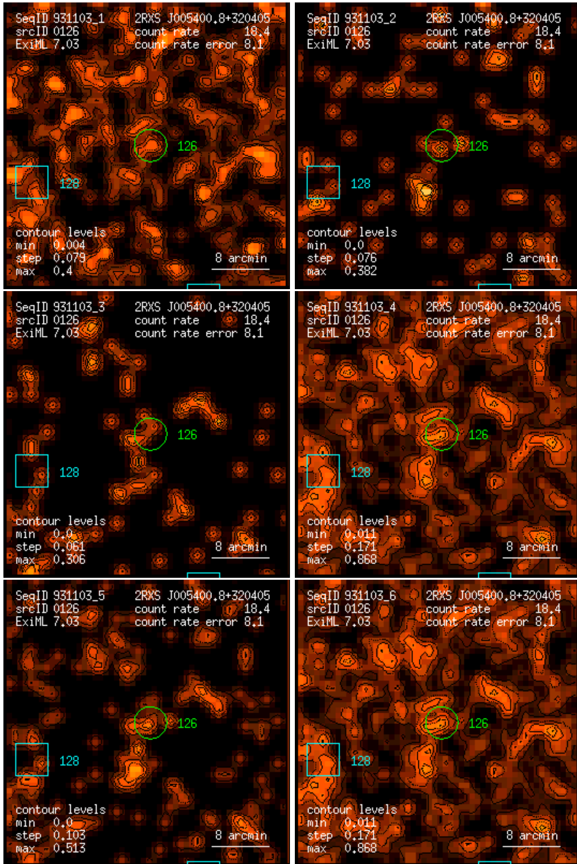
Figure 126: RASS 931103: detection 0126: band rate images, Gaussian filter: (1) PSPC channels 11 – 41, (2) 52 – 90, (3) 91 – 201, (4) 11 – 235, (5) 52 – 201, (6) 11 – 201. Broad band rates in counts/ks. Band rate contour levels in counts/ks/arcmin 2 .
