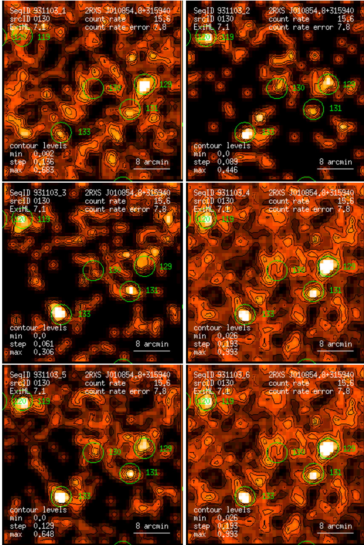
Figure 130: RASS 931103: detection 0130: band rate images, Gaussian filter: (1) PSPC channels 11 – 41, (2) 52 – 90, (3) 91 – 201, (4) 11 – 235, (5) 52 – 201, (6) 11 – 201. Broad band rates in counts/ks. Band rate contour levels in counts/ks/arcmin 2 .
