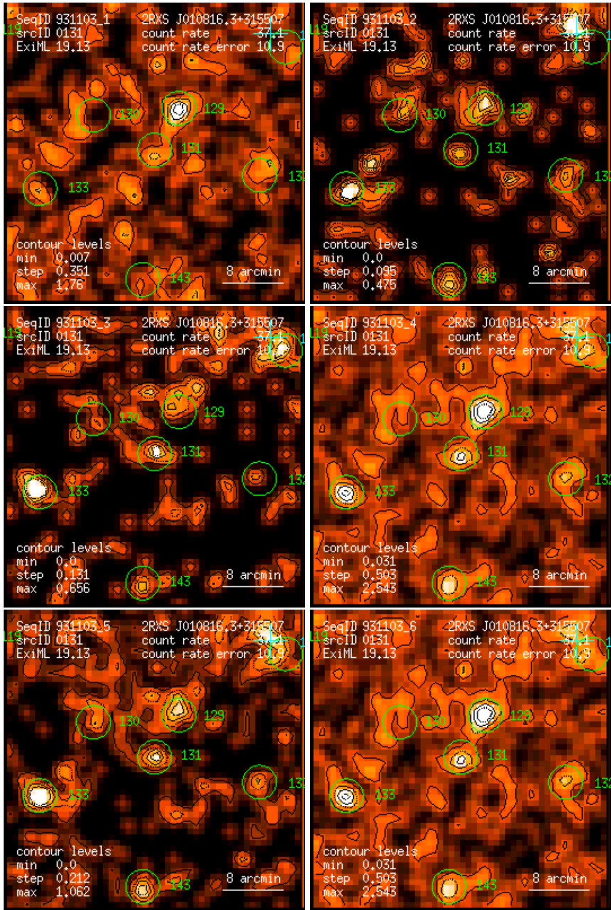
Figure 131: RASS 931103: detection 0131: band rate images, Gaussian filter: (1) PSPC channels 11 – 41, (2) 52 – 90, (3) 91 – 201, (4) 11 – 235, (5) 52 – 201, (6) 11 – 201. Broad band rates in counts/ks. Band rate contour levels in counts/ks/arcmin 2 .
