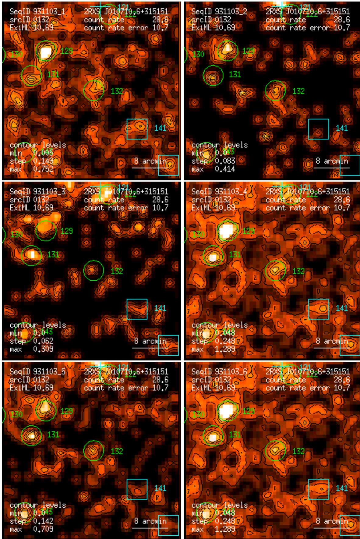
Figure 132: RASS 931103: detection 0132: band rate images, Gaussian filter: (1) PSPC channels 11 – 41, (2) 52 – 90, (3) 91 – 201, (4) 11 – 235, (5) 52 – 201, (6) 11 – 201. Broad band rates in counts/ks. Band rate contour levels in counts/ks/arcmin 2 .
