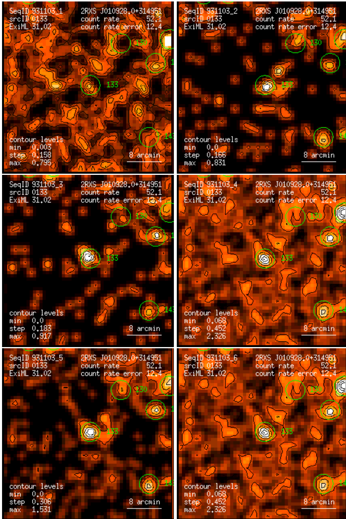
Figure 133: RASS 931103: detection 0133: band rate images, Gaussian filter: (1) PSPC channels 11 – 41, (2) 52 – 90, (3) 91 – 201, (4) 11 – 235, (5) 52 – 201, (6) 11 – 201. Broad band rates in counts/ks. Band rate contour levels in counts/ks/arcmin 2 .
