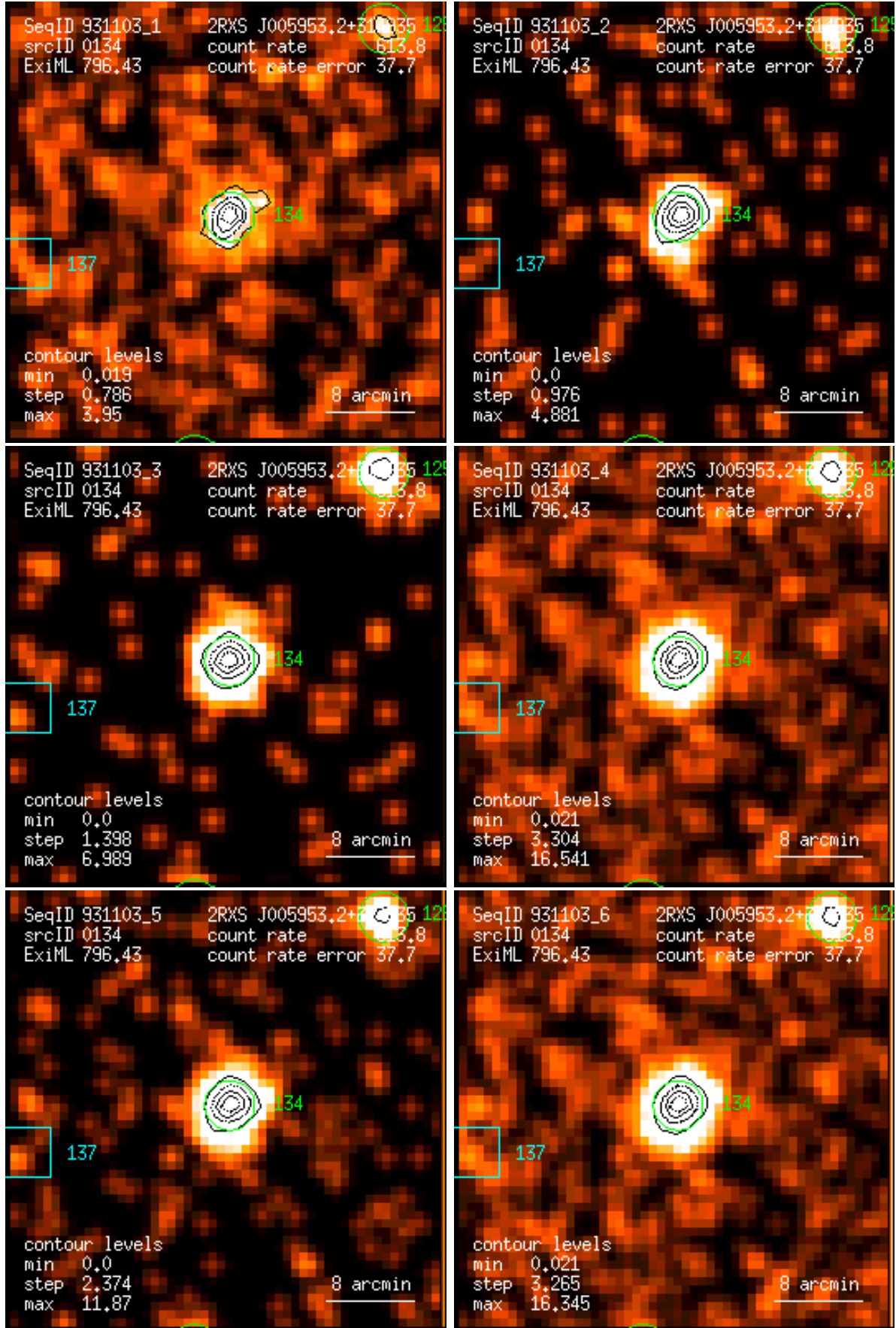
Figure 134: RASS 931103: detection 0134: band rate images, Gaussian filter: (1) PSPC channels 11 – 41, (2) 52 – 90, (3) 91 – 201, (4) 11 – 235, (5) 52 – 201, (6) 11 – 201. Broad band rates in counts/ks. Band rate contour levels in counts/ks/arcmin 2 .
