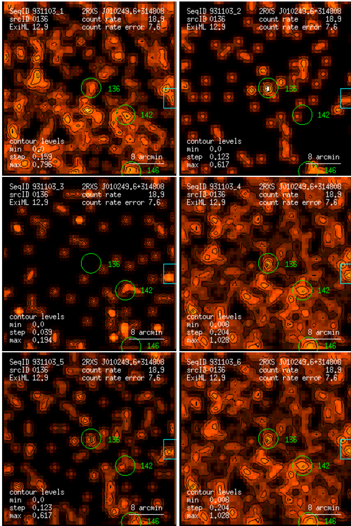
Figure 136: RASS 931103: detection 0136: band rate images, Gaussian filter: (1) PSPC channels 11 – 41, (2) 52 – 90, (3) 91 – 201, (4) 11 – 235, (5) 52 – 201, (6) 11 – 201. Broad band rates in counts/ks. Band rate contour levels in counts/ks/arcmin 2 .
