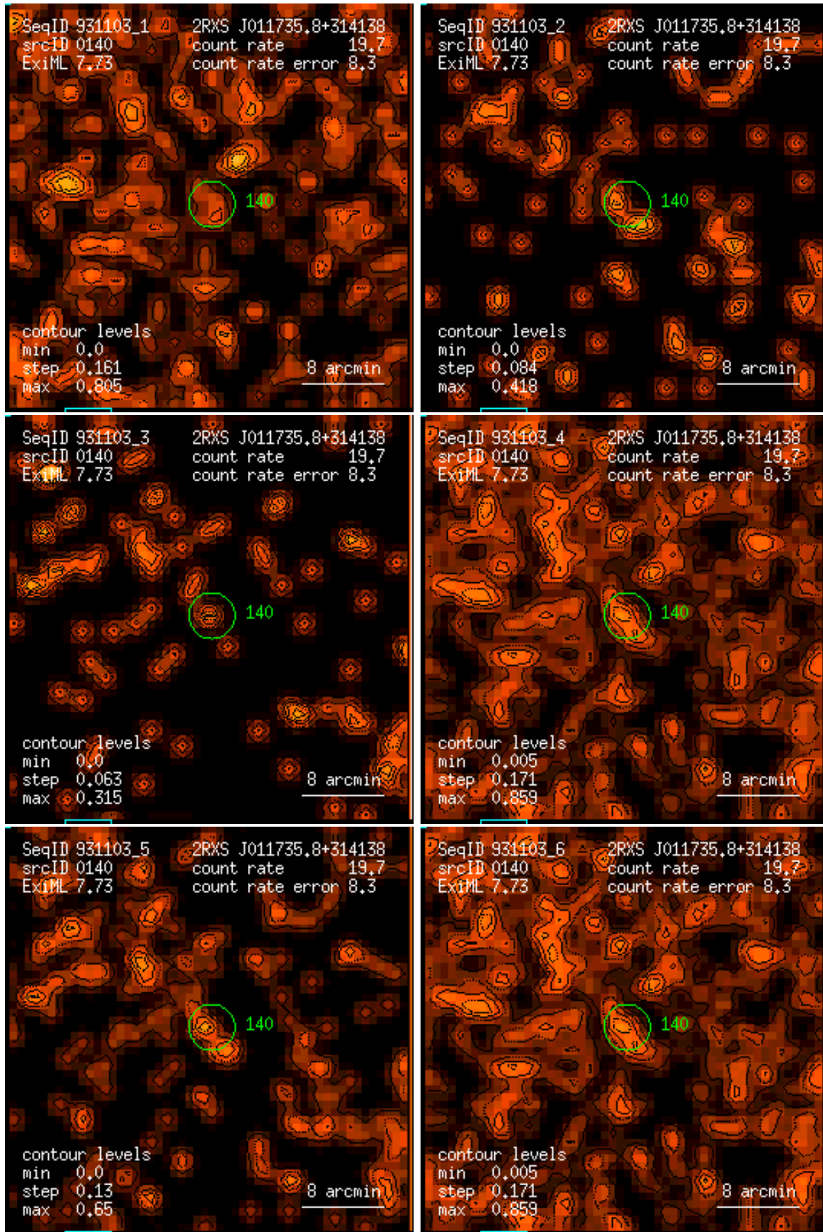
Figure 140: RASS 931103: detection 0140: band rate images, Gaussian filter: (1) PSPC channels 11 – 41, (2) 52 – 90, (3) 91 – 201, (4) 11 – 235, (5) 52 – 201, (6) 11 – 201. Broad band rates in counts/ks. Band rate contour levels in counts/ks/arcmin 2 .
