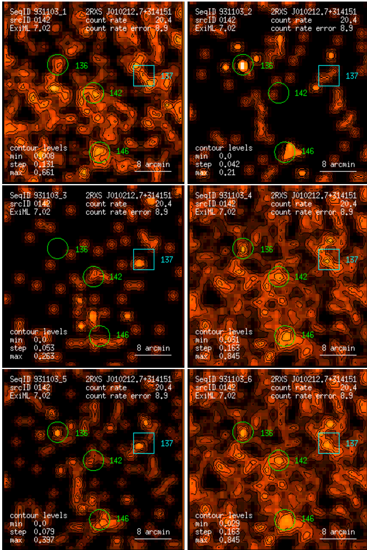
Figure 142: RASS 931103: detection 0142: band rate images, Gaussian filter: (1) PSPC channels 11 – 41, (2) 52 – 90, (3) 91 – 201, (4) 11 – 235, (5) 52 – 201, (6) 11 – 201. Broad band rates in counts/ks. Band rate contour levels in counts/ks/arcmin 2 .
