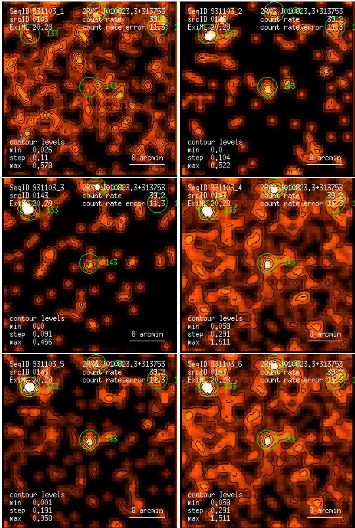
Figure 143: RASS 931103: detection 0143: band rate images, Gaussian filter: (1) PSPC channels 11 – 41, (2) 52 – 90, (3) 91 – 201, (4) 11 – 235, (5) 52 – 201, (6) 11 – 201. Broad band rates in counts/ks. Band rate contour levels in counts/ks/arcmin 2 .
