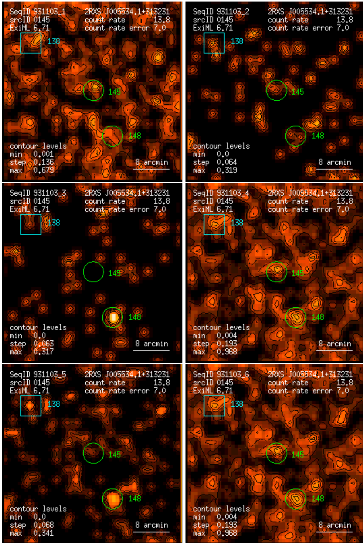
Figure 145: RASS 931103: detection 0145: band rate images, Gaussian filter: (1) PSPC channels 11 – 41, (2) 52 – 90, (3) 91 – 201, (4) 11 – 235, (5) 52 – 201, (6) 11 – 201. Broad band rates in counts/ks. Band rate contour levels in counts/ks/arcmin 2 .
