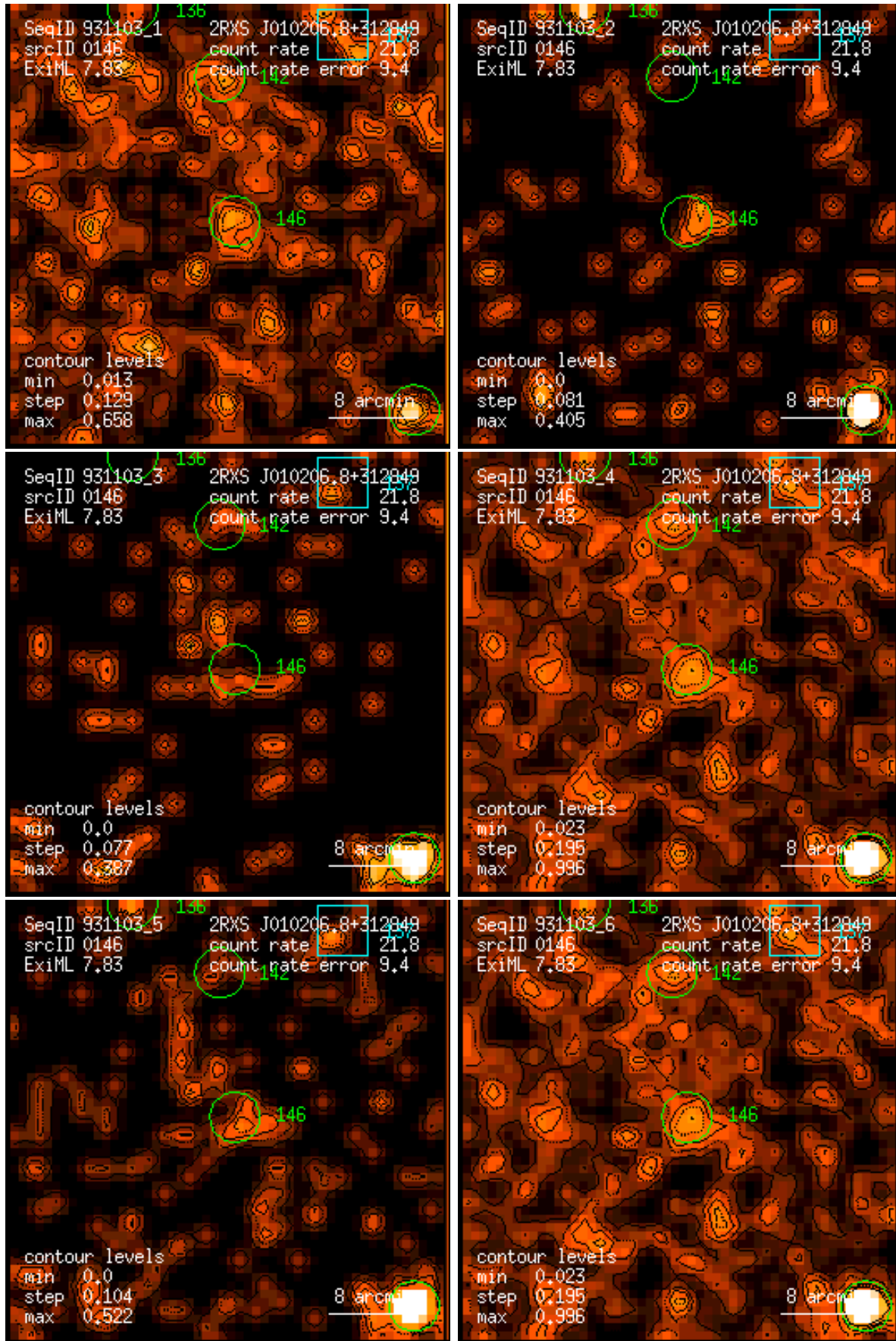
Figure 146: RASS 931103: detection 0146: band rate images, Gaussian filter: (1) PSPC channels 11 – 41, (2) 52 – 90, (3) 91 – 201, (4) 11 – 235, (5) 52 – 201, (6) 11 – 201. Broad band rates in counts/ks. Band rate contour levels in counts/ks/arcmin 2 .
