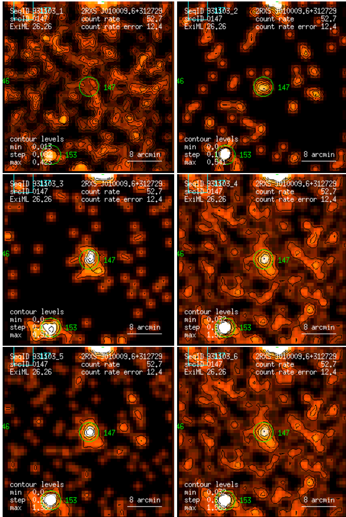
Figure 147: RASS 931103: detection 0147: band rate images, Gaussian filter: (1) PSPC channels 11 – 41, (2) 52 – 90, (3) 91 – 201, (4) 11 – 235, (5) 52 – 201, (6) 11 – 201. Broad band rates in counts/ks. Band rate contour levels in counts/ks/arcmin 2 .
