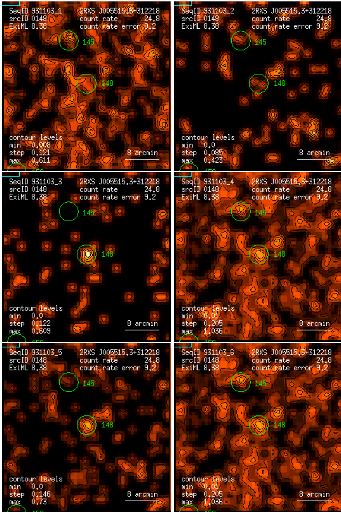
Figure 148: RASS 931103: detection 0148: band rate images, Gaussian filter: (1) PSPC channels 11 – 41, (2) 52 – 90, (3) 91 – 201, (4) 11 – 235, (5) 52 – 201, (6) 11 – 201. Broad band rates in counts/ks. Band rate contour levels in counts/ks/arcmin 2 .
