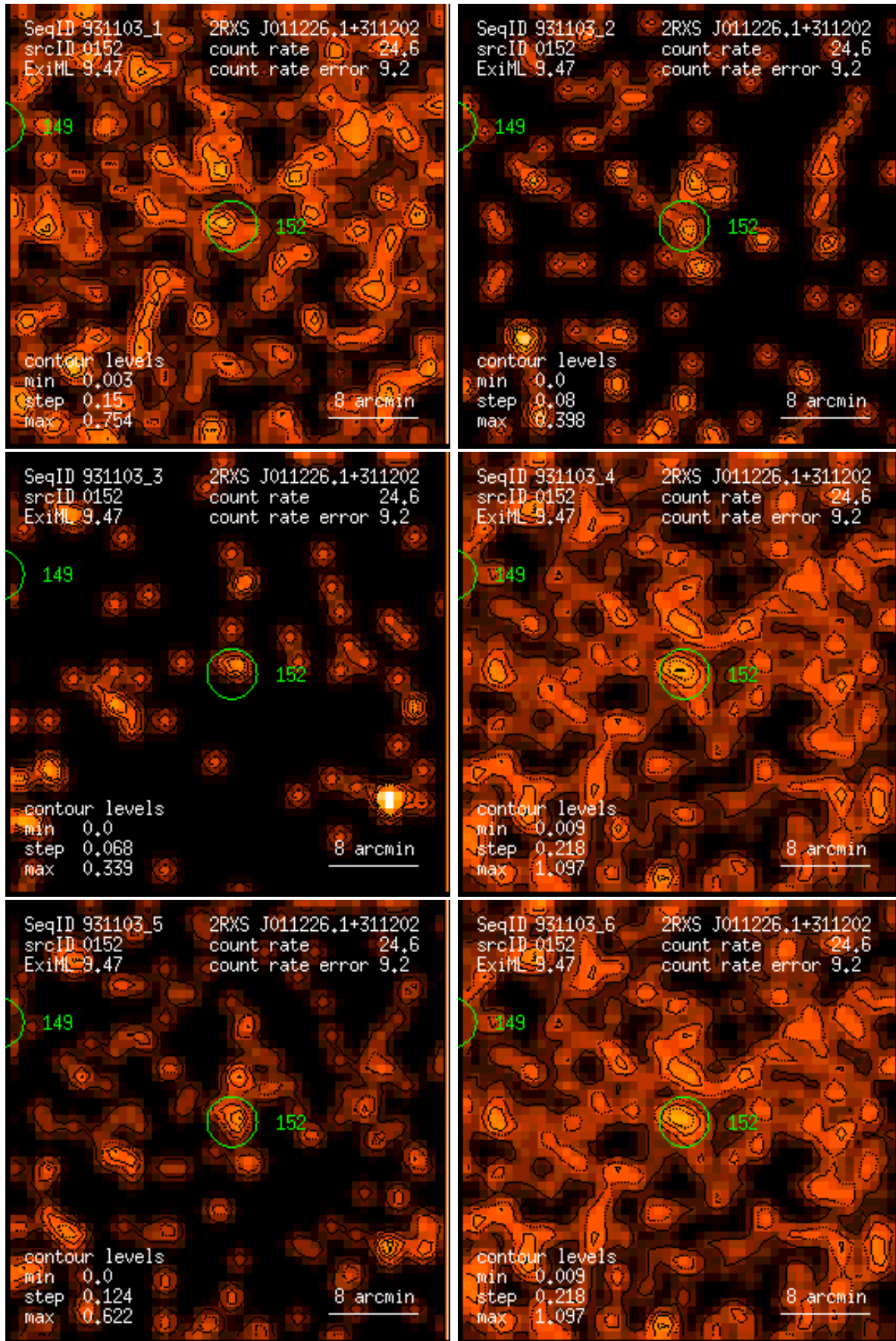
Figure 152: RASS 931103: detection 0152: band rate images, Gaussian filter: (1) PSPC channels 11 – 41, (2) 52 – 90, (3) 91 – 201, (4) 11 – 235, (5) 52 – 201, (6) 11 – 201. Broad band rates in counts/ks. Band rate contour levels in counts/ks/arcmin 2 .
