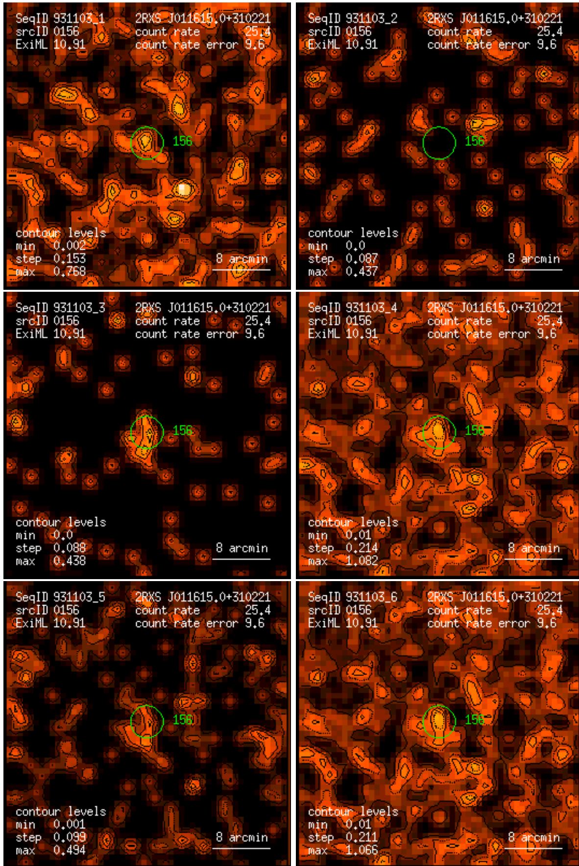
Figure 156: RASS 931103: detection 0156: band rate images, Gaussian filter: (1) PSPC channels 11 – 41, (2) 52 – 90, (3) 91 – 201, (4) 11 – 235, (5) 52 – 201, (6) 11 – 201. Broad band rates in counts/ks. Band rate contour levels in counts/ks/arcmin 2 .
