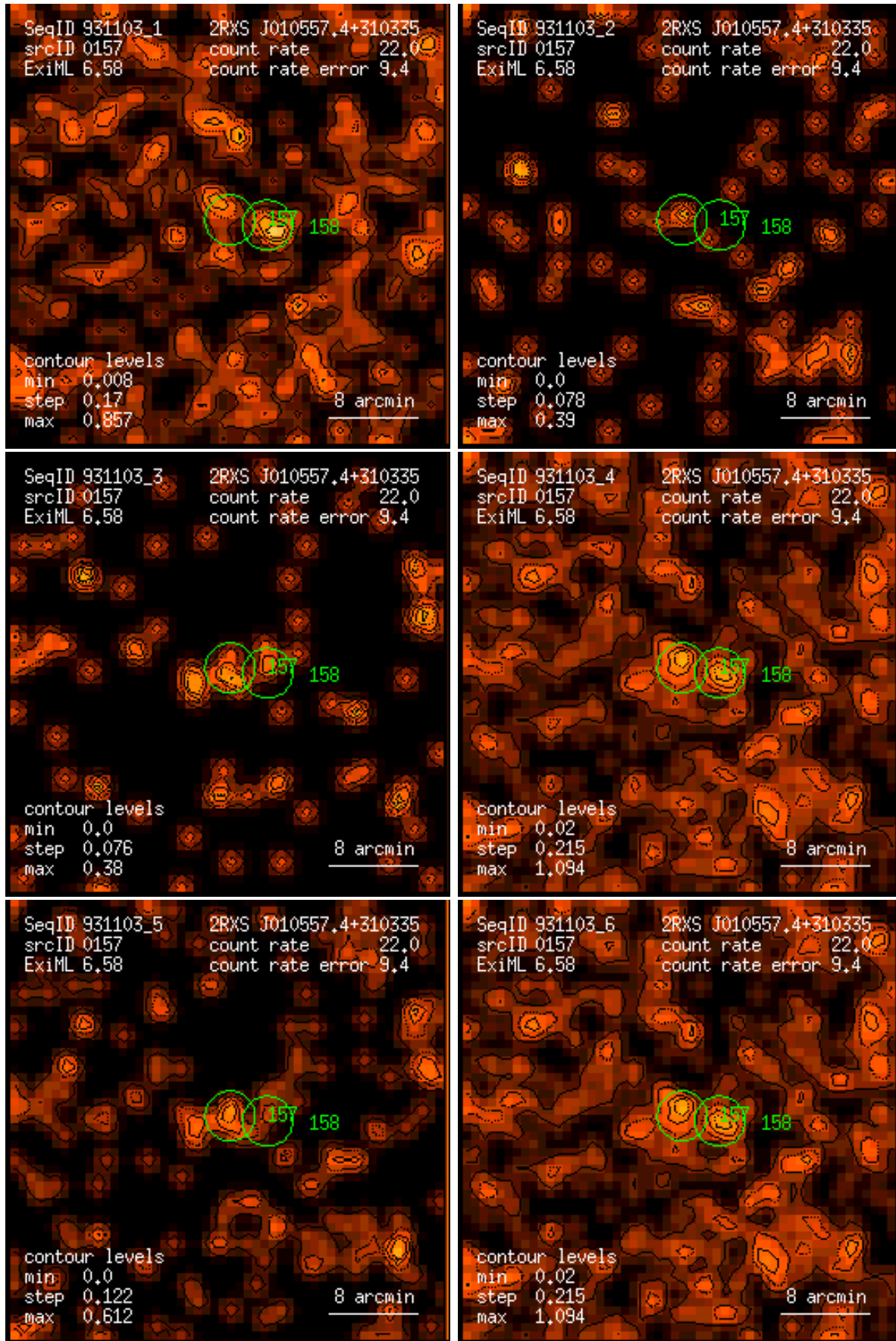
Figure 157: RASS 931103: detection 0157: band rate images, Gaussian filter: (1) PSPC channels 11 – 41, (2) 52 – 90, (3) 91 – 201, (4) 11 – 235, (5) 52 – 201, (6) 11 – 201. Broad band rates in counts/ks. Band rate contour levels in counts/ks/arcmin 2 .
