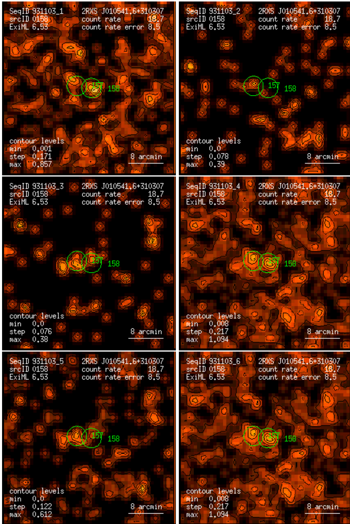
Figure 158: RASS 931103: detection 0158: band rate images, Gaussian filter: (1) PSPC channels 11 – 41, (2) 52 – 90, (3) 91 – 201, (4) 11 – 235, (5) 52 – 201, (6) 11 – 201. Broad band rates in counts/ks. Band rate contour levels in counts/ks/arcmin 2 .
