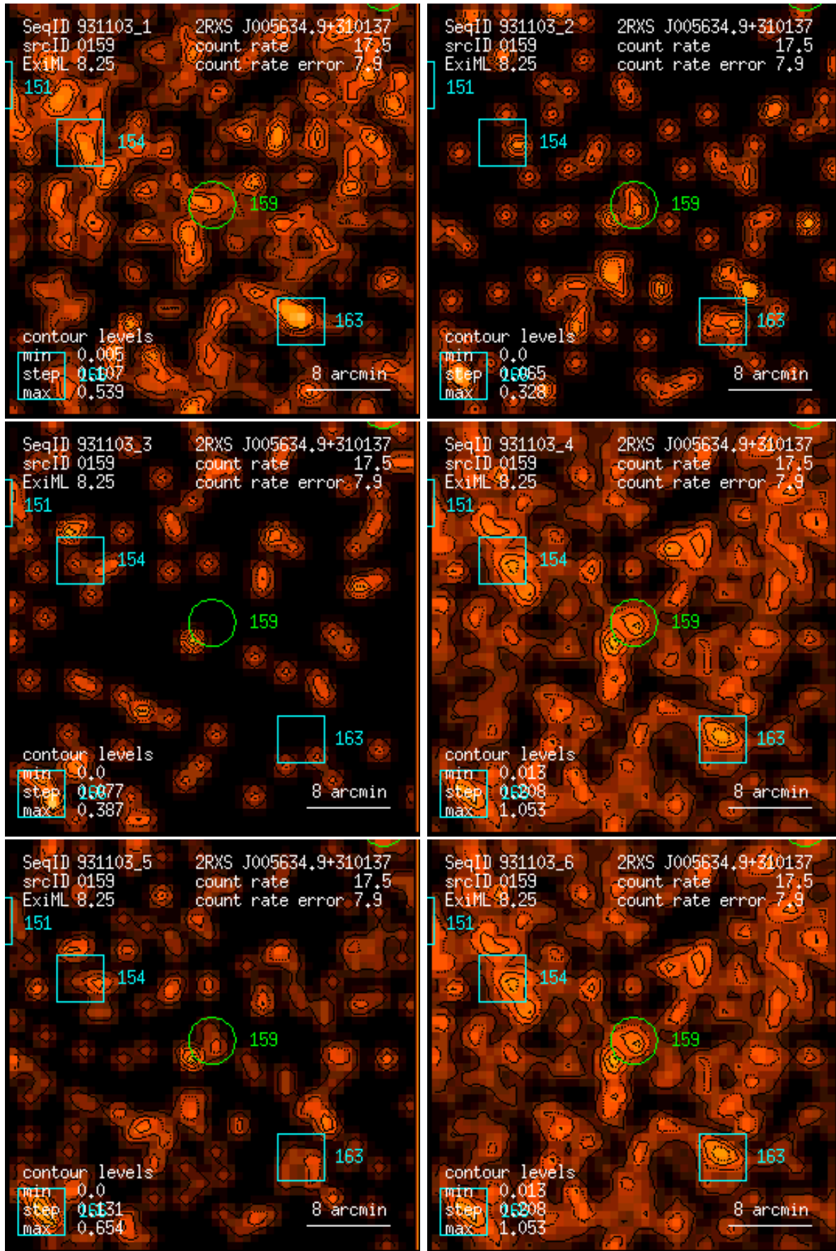
Figure 159: RASS 931103: detection 0159: band rate images, Gaussian filter: (1) PSPC channels 11 – 41, (2) 52 – 90, (3) 91 – 201, (4) 11 – 235, (5) 52 – 201, (6) 11 – 201. Broad band rates in counts/ks. Band rate contour levels in counts/ks/arcmin 2 .
