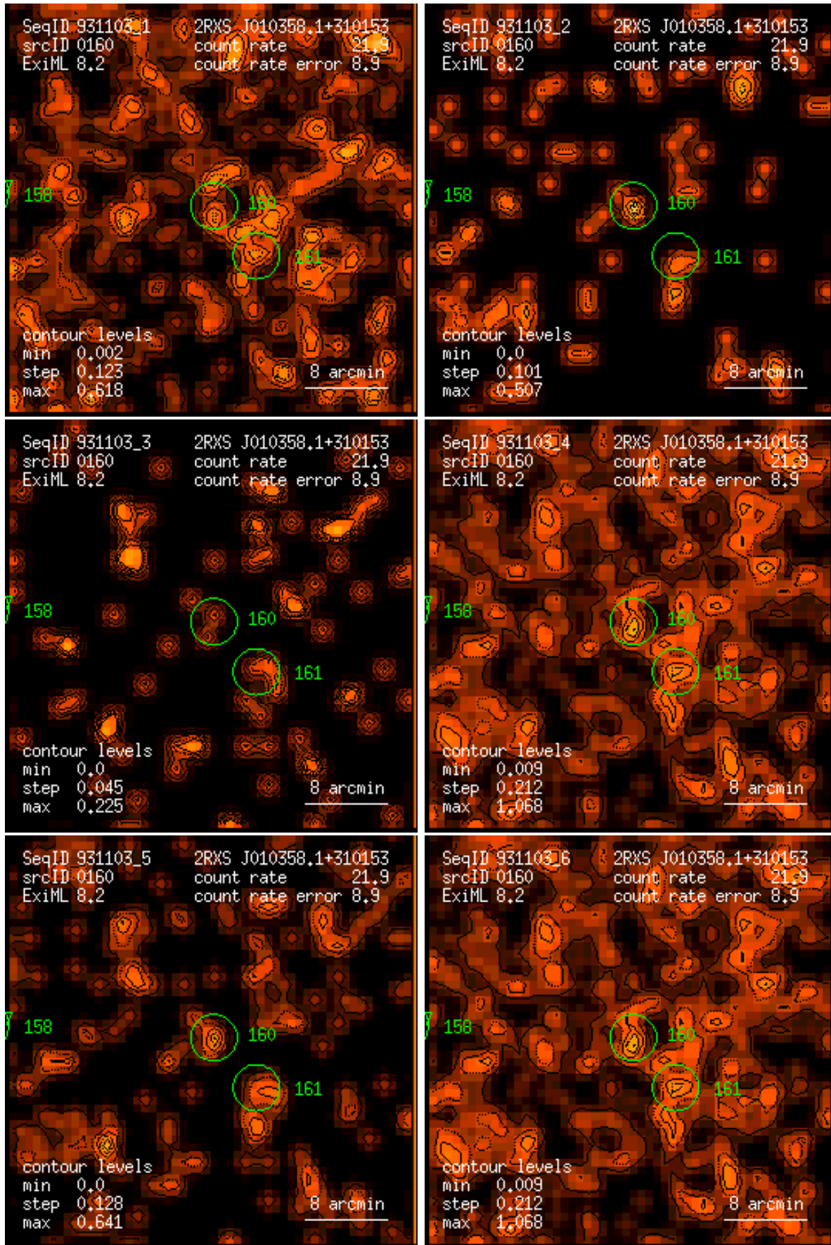
Figure 160: RASS 931103: detection 0160: band rate images, Gaussian filter: (1) PSPC channels 11 – 41, (2) 52 – 90, (3) 91 – 201, (4) 11 – 235, (5) 52 – 201, (6) 11 – 201. Broad band rates in counts/ks. Band rate contour levels in counts/ks/arcmin 2 .
