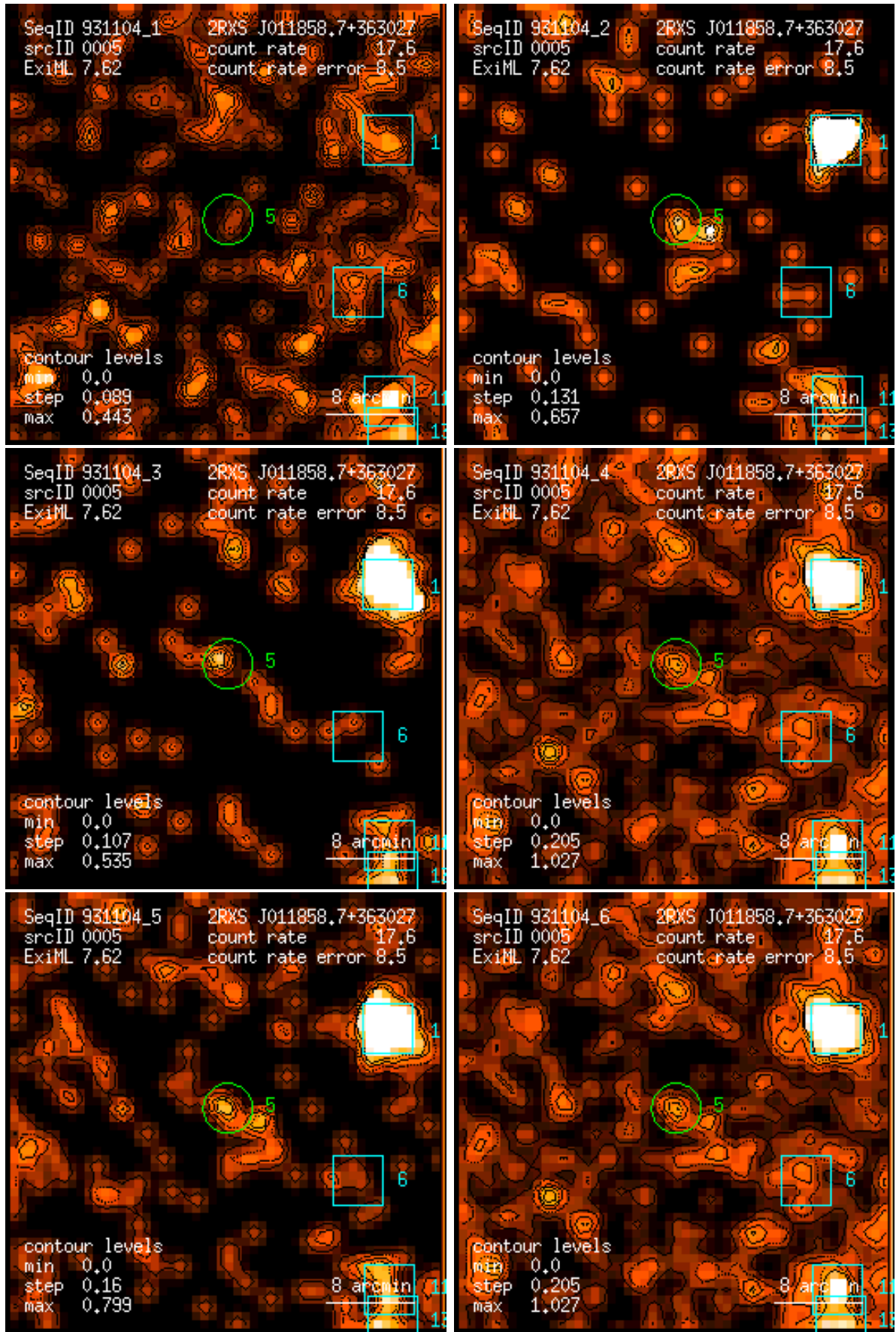
Figure 5: RASS 931104: detection 0005: band rate images, Gaussian filter: (1) PSPC channels 11 – 41, (2) 52 – 90, (3) 91 – 201, (4) 11 – 235, (5) 52 – 201, (6) 11 – 201. Broad band rates in counts/ks. Band rate contour levels in counts/ks/arcmin 2 .
