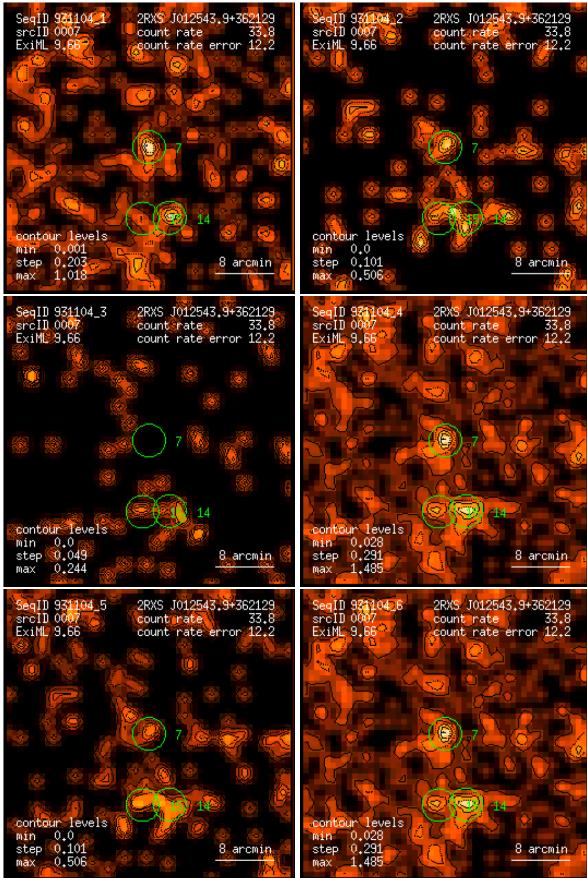
Figure 7: RASS 931104: detection 0007: band rate images, Gaussian filter: (1) PSPC channels 11 – 41, (2) 52 – 90, (3) 91 – 201, (4) 11 – 235, (5) 52 – 201, (6) 11 – 201. Broad band rates in counts/ks. Band rate contour levels in counts/ks/arcmin 2 .
