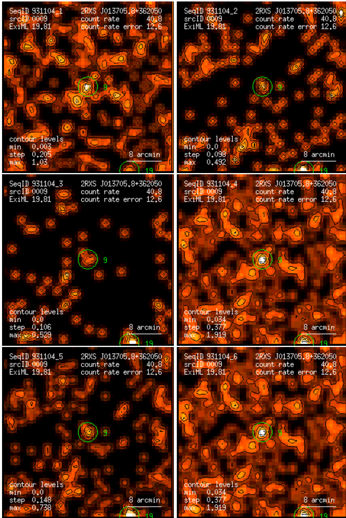
Figure 9: RASS 931104: detection 0009: band rate images, Gaussian filter: (1) PSPC channels 11 – 41, (2) 52 – 90, (3) 91 – 201, (4) 11 – 235, (5) 52 – 201, (6) 11 – 201. Broad band rates in counts/ks. Band rate contour levels in counts/ks/arcmin 2 .
