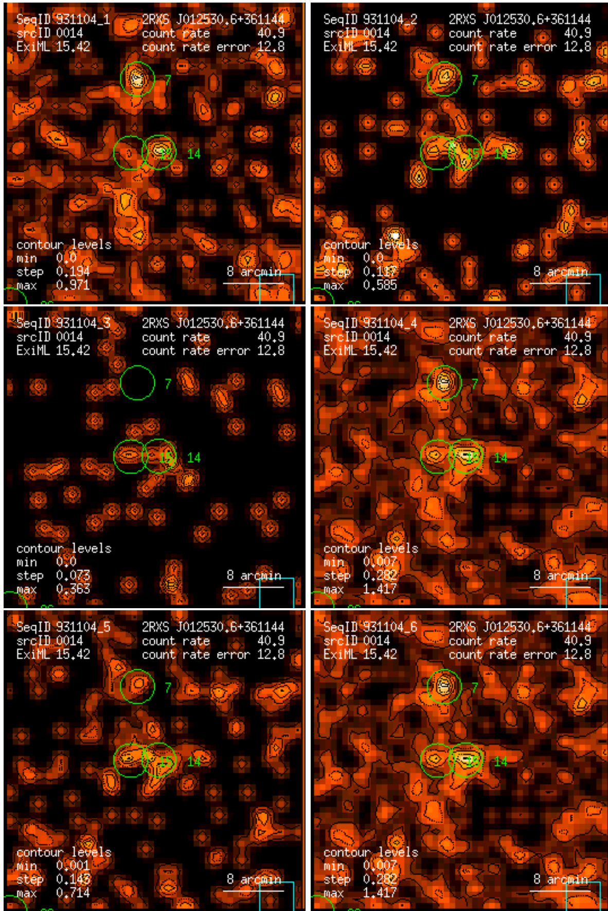
Figure 14: RASS 931104: detection 0014: band rate images, Gaussian filter: (1) PSPC channels 11 – 41, (2) 52 – 90, (3) 91 – 201, (4) 11 – 235, (5) 52 – 201, (6) 11 – 201. Broad band rates in counts/ks. Band rate contour levels in counts/ks/arcmin 2 .
