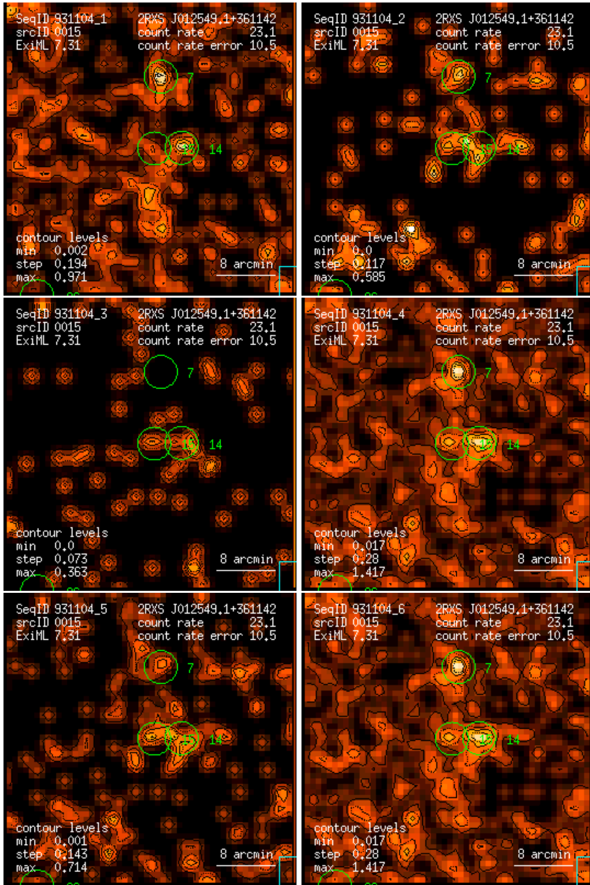
Figure 15: RASS 931104: detection 0015: band rate images, Gaussian filter: (1) PSPC channels 11 – 41, (2) 52 – 90, (3) 91 – 201, (4) 11 – 235, (5) 52 – 201, (6) 11 – 201. Broad band rates in counts/ks. Band rate contour levels in counts/ks/arcmin 2 .
