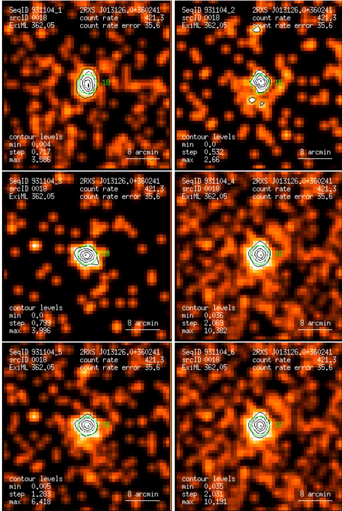
Figure 18: RASS 931104: detection 0018: band rate images, Gaussian filter: (1) PSPC channels 11 – 41, (2) 52 – 90, (3) 91 – 201, (4) 11 – 235, (5) 52 – 201, (6) 11 – 201. Broad band rates in counts/ks. Band rate contour levels in counts/ks/arcmin 2 .
