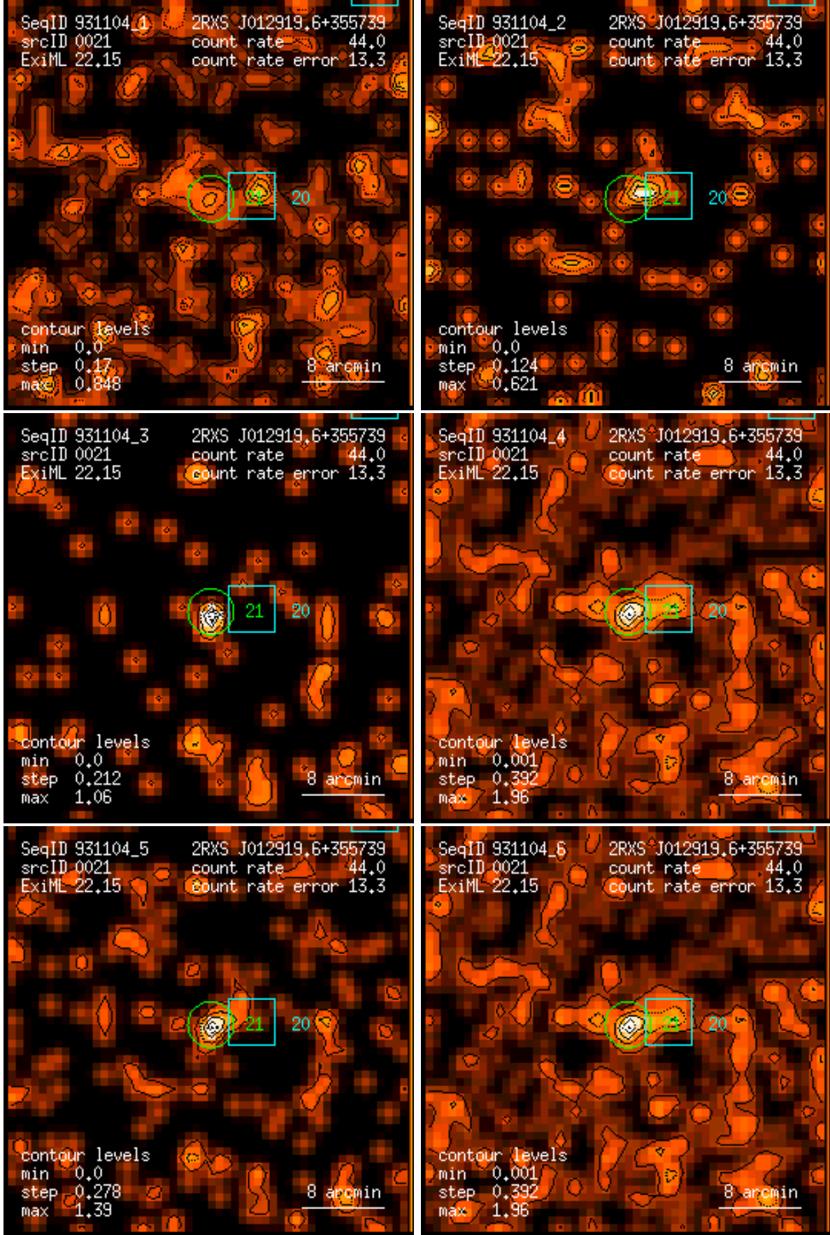
Figure 21: RASS 931104: detection 0021: band rate images, Gaussian filter: (1) PSPC channels 11 – 41, (2) 52 – 90, (3) 91 – 201, (4) 11 – 235, (5) 52 – 201, (6) 11 – 201. Broad band rates in counts/ks. Band rate contour levels in counts/ks/arcmin 2 .
