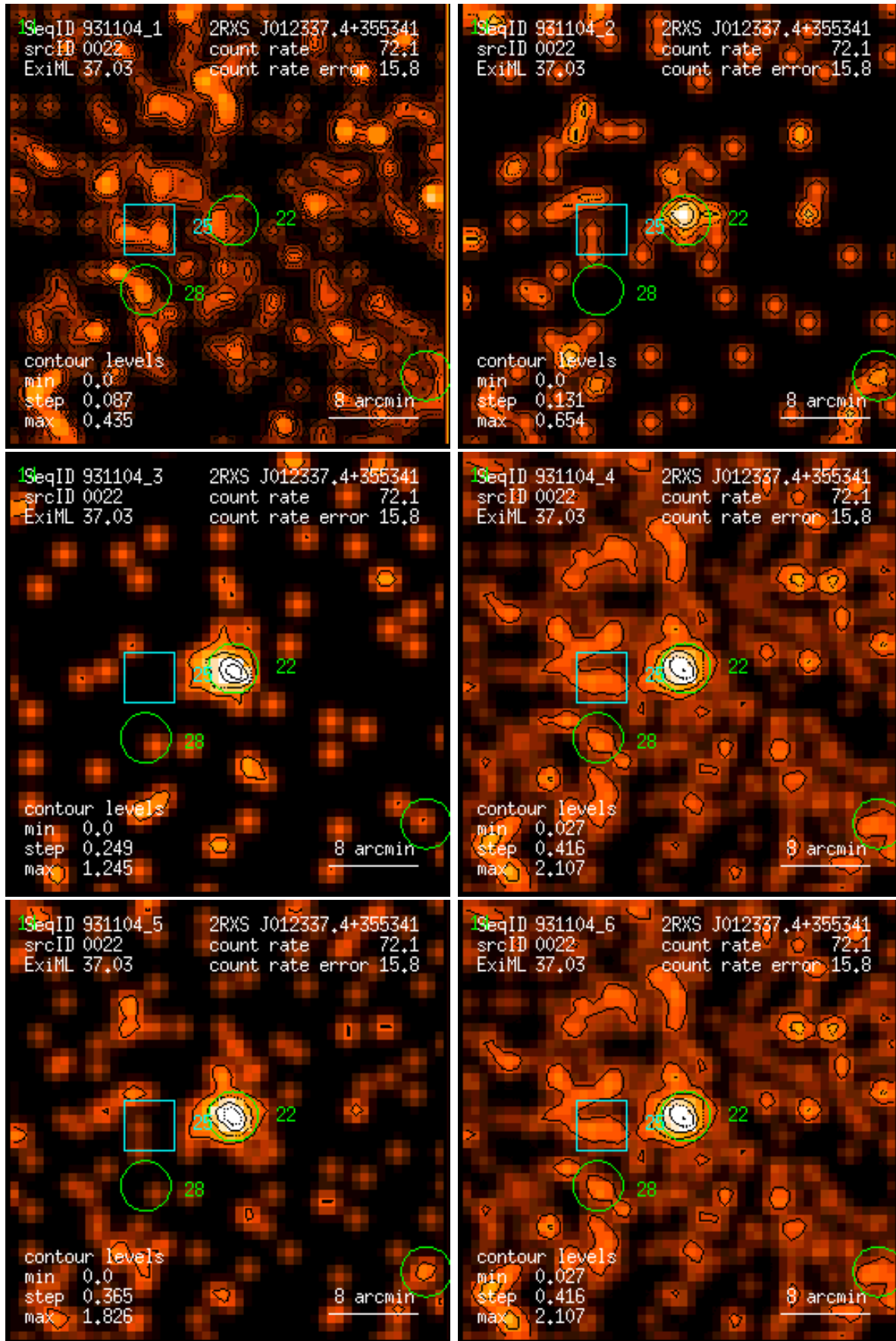
Figure 22: RASS 931104: detection 0022: band rate images, Gaussian filter: (1) PSPC channels 11 – 41, (2) 52 – 90, (3) 91 – 201, (4) 11 – 235, (5) 52 – 201, (6) 11 – 201. Broad band rates in counts/ks. Band rate contour levels in counts/ks/arcmin 2 .
