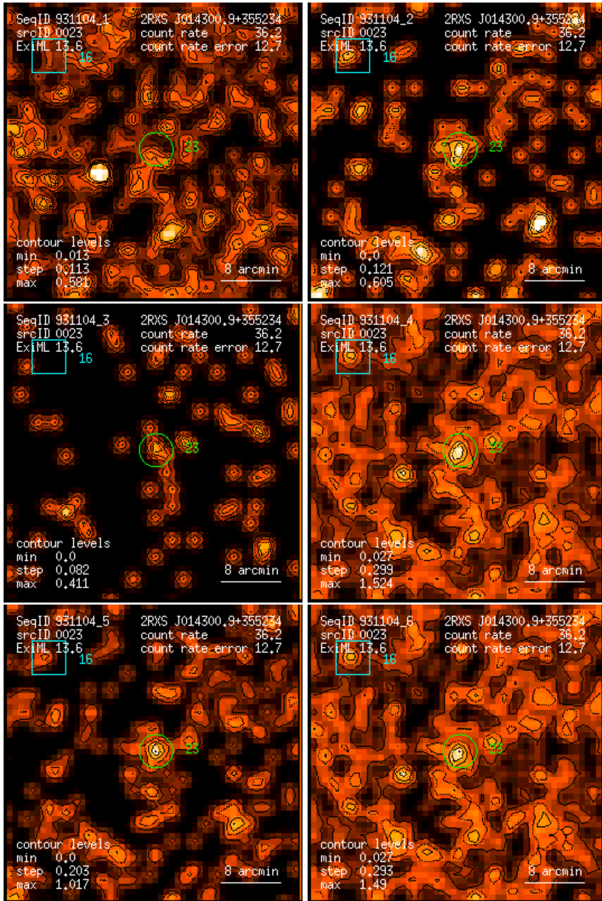
Figure 23: RASS 931104: detection 0023: band rate images, Gaussian filter: (1) PSPC channels 11 – 41, (2) 52 – 90, (3) 91 – 201, (4) 11 – 235, (5) 52 – 201, (6) 11 – 201. Broad band rates in counts/ks. Band rate contour levels in counts/ks/arcmin 2 .
