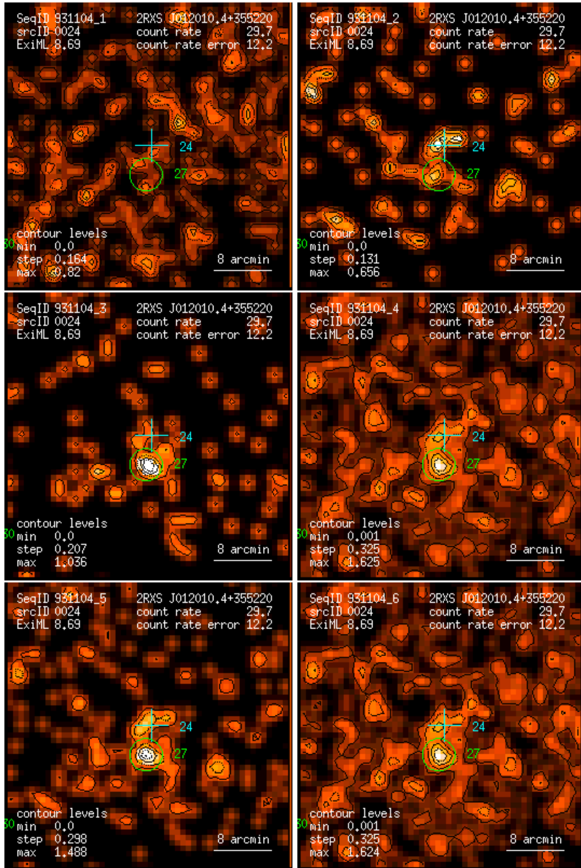
Figure 24: RASS 931104: detection 0024: band rate images, Gaussian filter: (1) PSPC channels 11 – 41, (2) 52 – 90, (3) 91 – 201, (4) 11 – 235, (5) 52 – 201, (6) 11 – 201. Broad band rates in counts/ks. Band rate contour levels in counts/ks/arcmin 2 .
