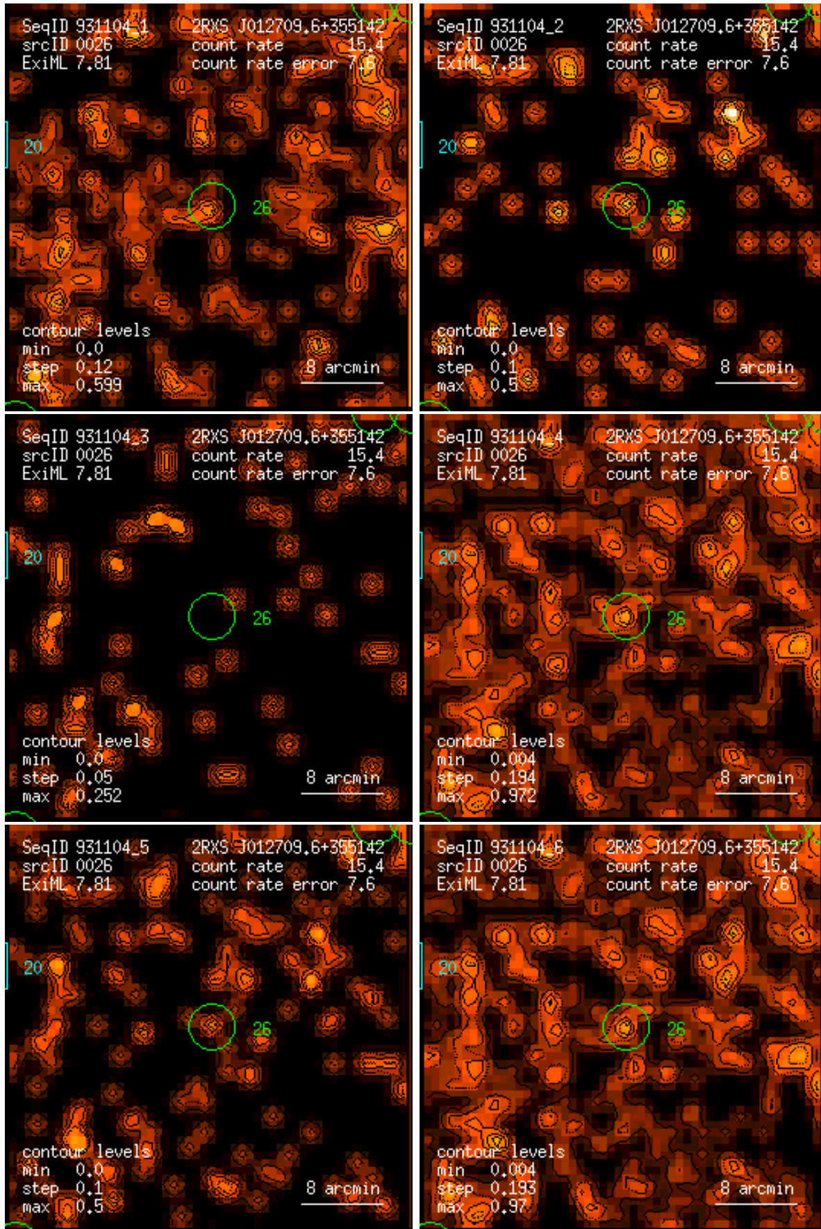
Figure 26: RASS 931104: detection 0026: band rate images, Gaussian filter: (1) PSPC channels 11 – 41, (2) 52 – 90, (3) 91 – 201, (4) 11 – 235, (5) 52 – 201, (6) 11 – 201. Broad band rates in counts/ks. Band rate contour levels in counts/ks/arcmin 2 .
