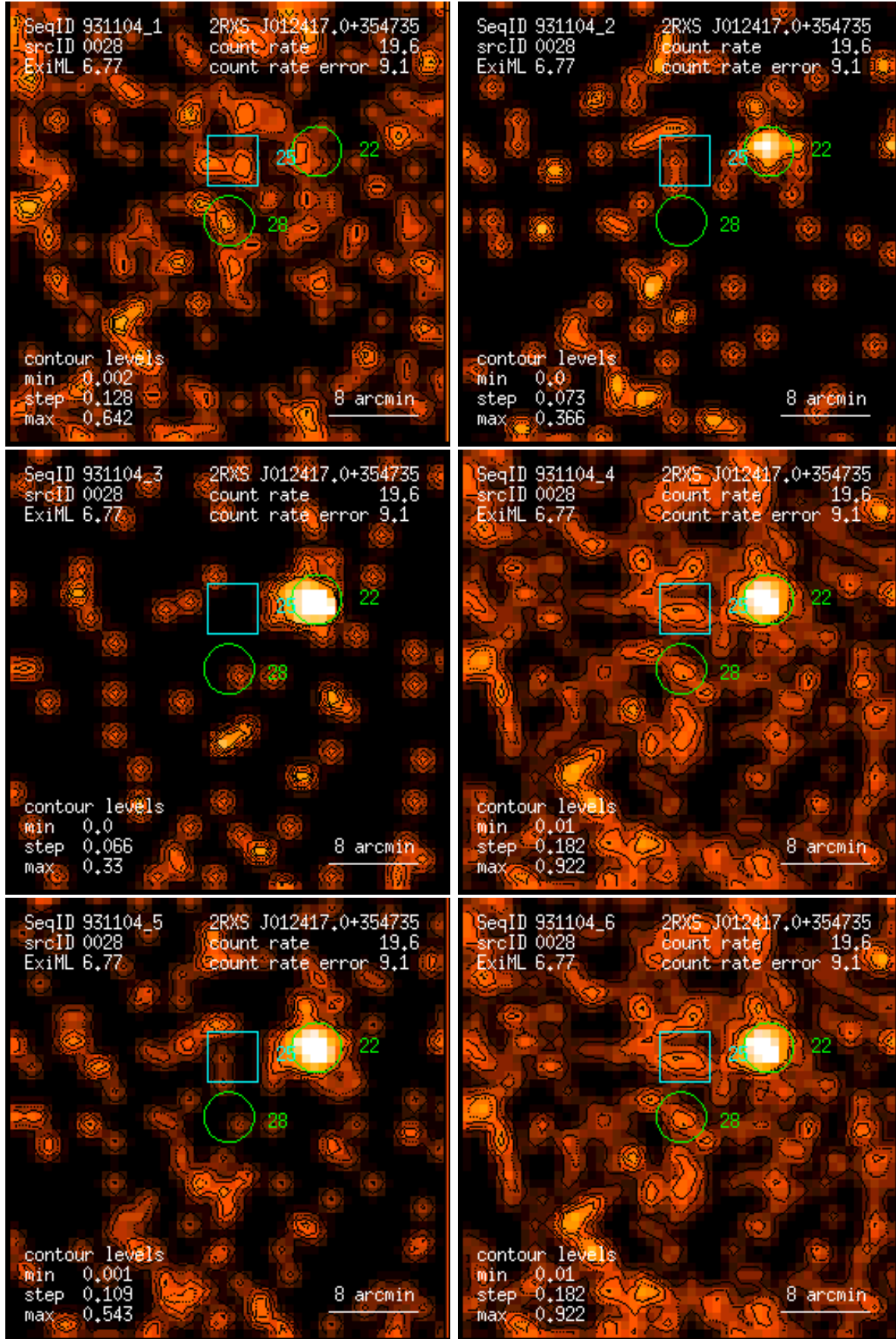
Figure 28: RASS 931104: detection 0028: band rate images, Gaussian filter: (1) PSPC channels 11 – 41, (2) 52 – 90, (3) 91 – 201, (4) 11 – 235, (5) 52 – 201, (6) 11 – 201. Broad band rates in counts/ks. Band rate contour levels in counts/ks/arcmin 2 .
