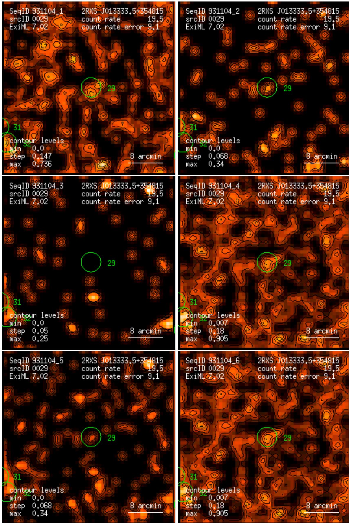
Figure 29: RASS 931104: detection 0029: band rate images, Gaussian filter: (1) PSPC channels 11 – 41, (2) 52 – 90, (3) 91 – 201, (4) 11 – 235, (5) 52 – 201, (6) 11 – 201. Broad band rates in counts/ks. Band rate contour levels in counts/ks/arcmin 2 .
