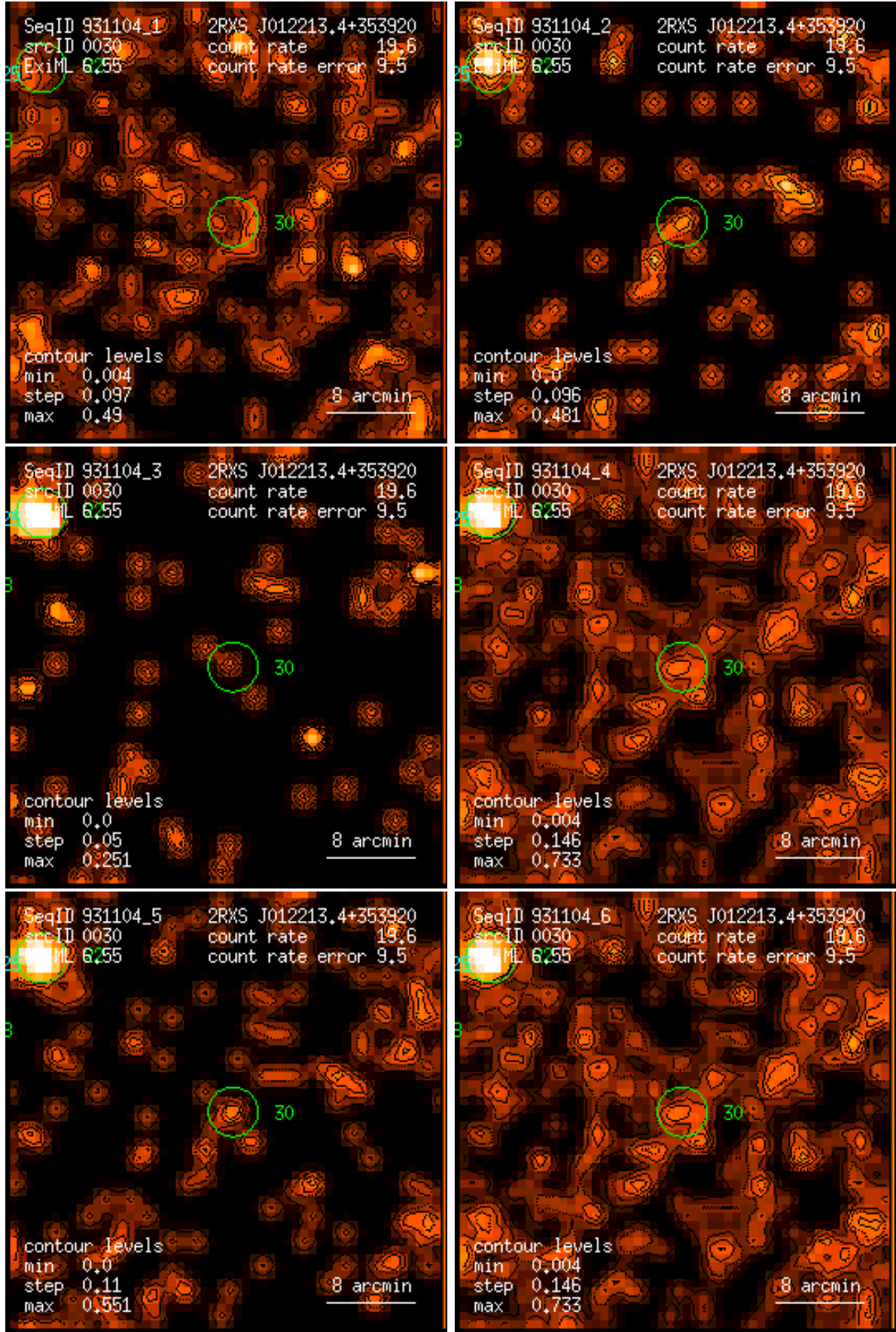
Figure 30: RASS 931104: detection 0030: band rate images, Gaussian filter: (1) PSPC channels 11 – 41, (2) 52 – 90, (3) 91 – 201, (4) 11 – 235, (5) 52 – 201, (6) 11 – 201. Broad band rates in counts/ks. Band rate contour levels in counts/ks/arcmin 2 .
