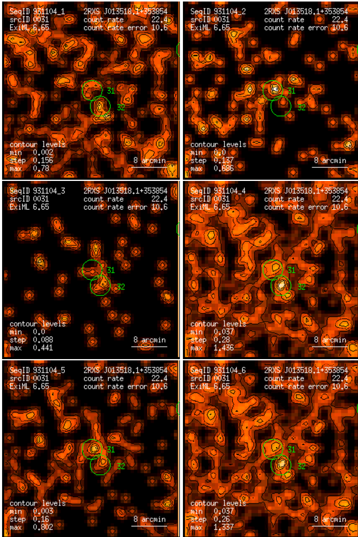
Figure 31: RASS 931104: detection 0031: band rate images, Gaussian filter: (1) PSPC channels 11 – 41, (2) 52 – 90, (3) 91 – 201, (4) 11 – 235, (5) 52 – 201, (6) 11 – 201. Broad band rates in counts/ks. Band rate contour levels in counts/ks/arcmin 2 .
