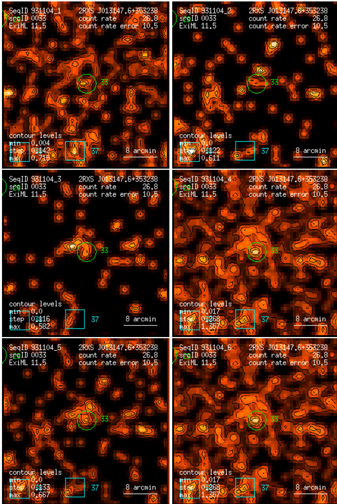
Figure 33: RASS 931104: detection 0033: band rate images, Gaussian filter: (1) PSPC channels 11 – 41, (2) 52 – 90, (3) 91 – 201, (4) 11 – 235, (5) 52 – 201, (6) 11 – 201. Broad band rates in counts/ks. Band rate contour levels in counts/ks/arcmin 2 .
