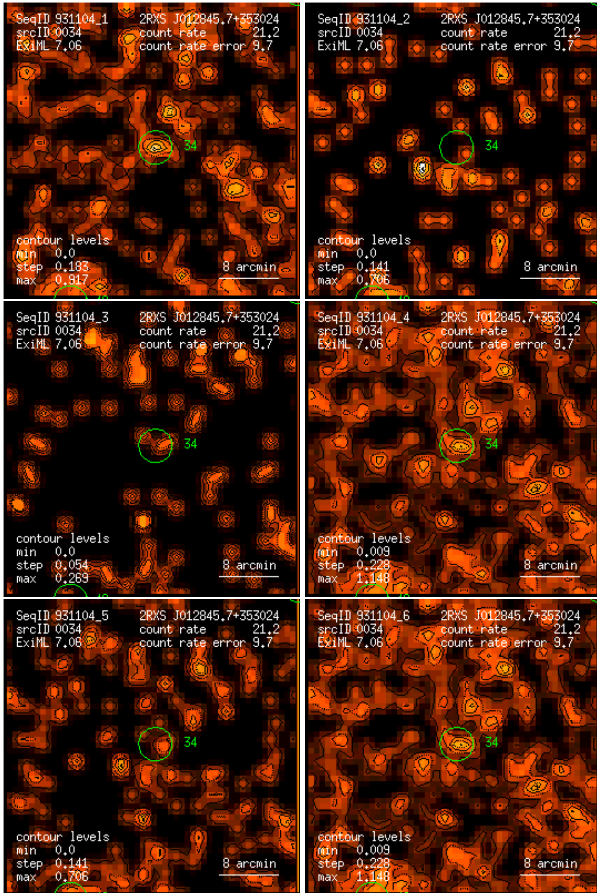
Figure 34: RASS 931104: detection 0034: band rate images, Gaussian filter: (1) PSPC channels 11 – 41, (2) 52 – 90, (3) 91 – 201, (4) 11 – 235, (5) 52 – 201, (6) 11 – 201. Broad band rates in counts/ks. Band rate contour levels in counts/ks/arcmin 2 .
