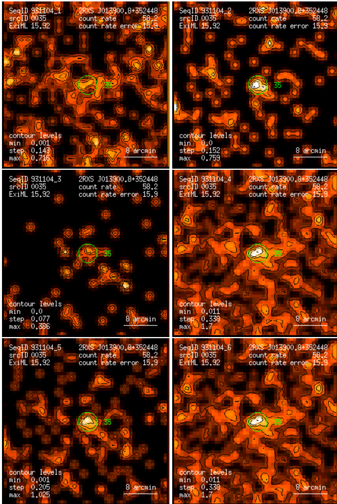
Figure 35: RASS 931104: detection 0035: band rate images, Gaussian filter: (1) PSPC channels 11 – 41, (2) 52 – 90, (3) 91 – 201, (4) 11 – 235, (5) 52 – 201, (6) 11 – 201. Broad band rates in counts/ks. Band rate contour levels in counts/ks/arcmin 2 .
