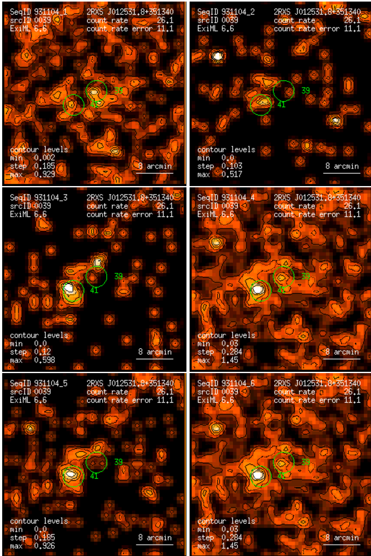
Figure 39: RASS 931104: detection 0039: band rate images, Gaussian filter: (1) PSPC channels 11 – 41, (2) 52 – 90, (3) 91 – 201, (4) 11 – 235, (5) 52 – 201, (6) 11 – 201. Broad band rates in counts/ks. Band rate contour levels in counts/ks/arcmin 2 .
