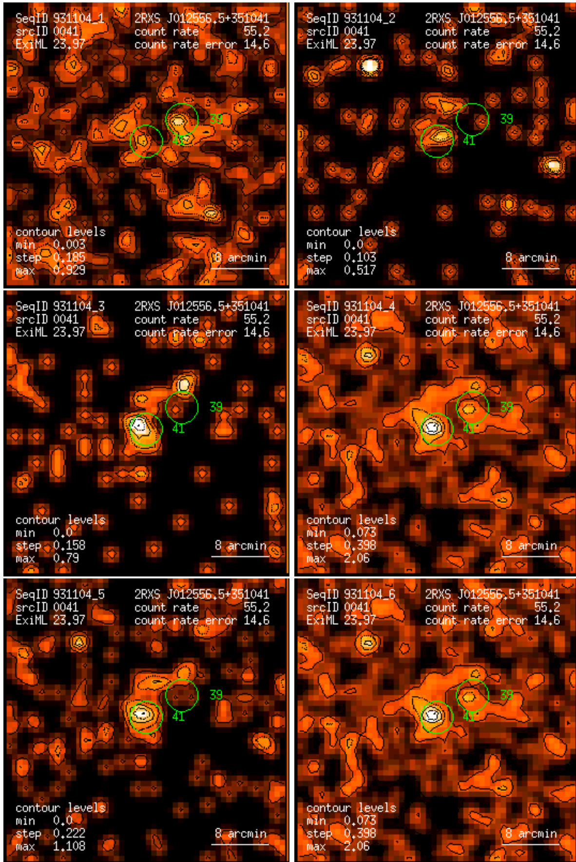
Figure 41: RASS 931104: detection 0041: band rate images, Gaussian filter: (1) PSPC channels 11 – 41, (2) 52 – 90, (3) 91 – 201, (4) 11 – 235, (5) 52 – 201, (6) 11 – 201. Broad band rates in counts/ks. Band rate contour levels in counts/ks/arcmin 2 .
