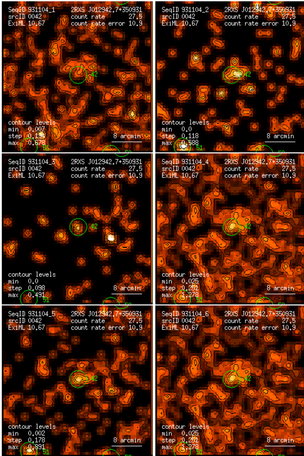
Figure 42: RASS 931104: detection 0042: band rate images, Gaussian filter: (1) PSPC channels 11 – 41, (2) 52 – 90, (3) 91 – 201, (4) 11 – 235, (5) 52 – 201, (6) 11 – 201. Broad band rates in counts/ks. Band rate contour levels in counts/ks/arcmin 2 .
