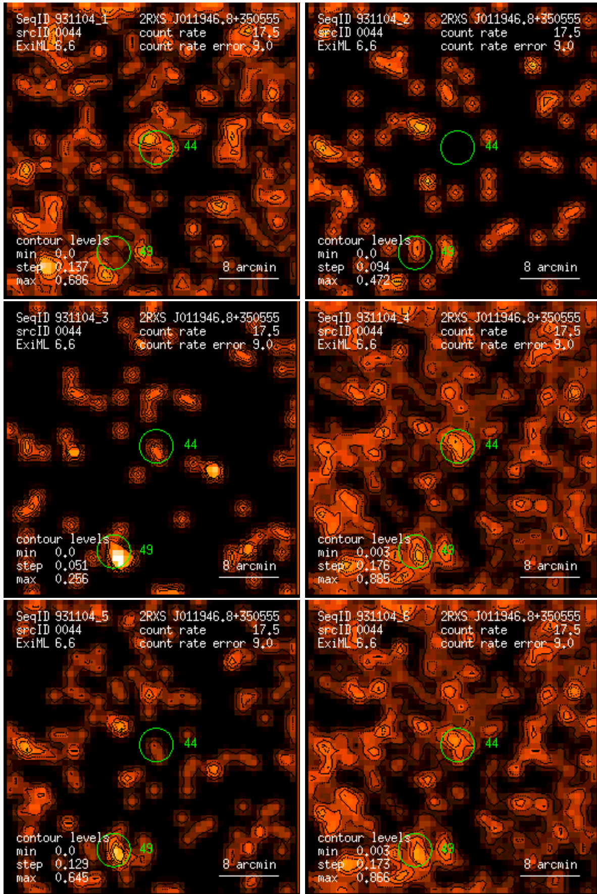
Figure 44: RASS 931104: detection 0044: band rate images, Gaussian filter: (1) PSPC channels 11 – 41, (2) 52 – 90, (3) 91 – 201, (4) 11 – 235, (5) 52 – 201, (6) 11 – 201. Broad band rates in counts/ks. Band rate contour levels in counts/ks/arcmin 2 .
