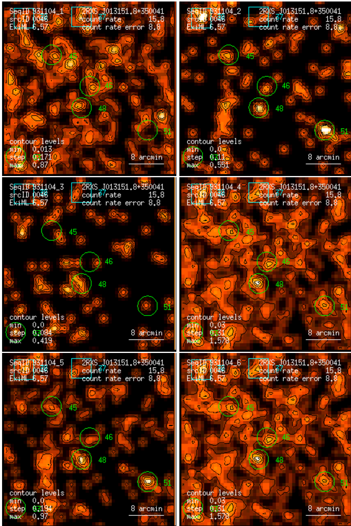
Figure 46: RASS 931104: detection 0046: band rate images, Gaussian filter: (1) PSPC channels 11 – 41, (2) 52 – 90, (3) 91 – 201, (4) 11 – 235, (5) 52 – 201, (6) 11 – 201. Broad band rates in counts/ks. Band rate contour levels in counts/ks/arcmin 2 .
