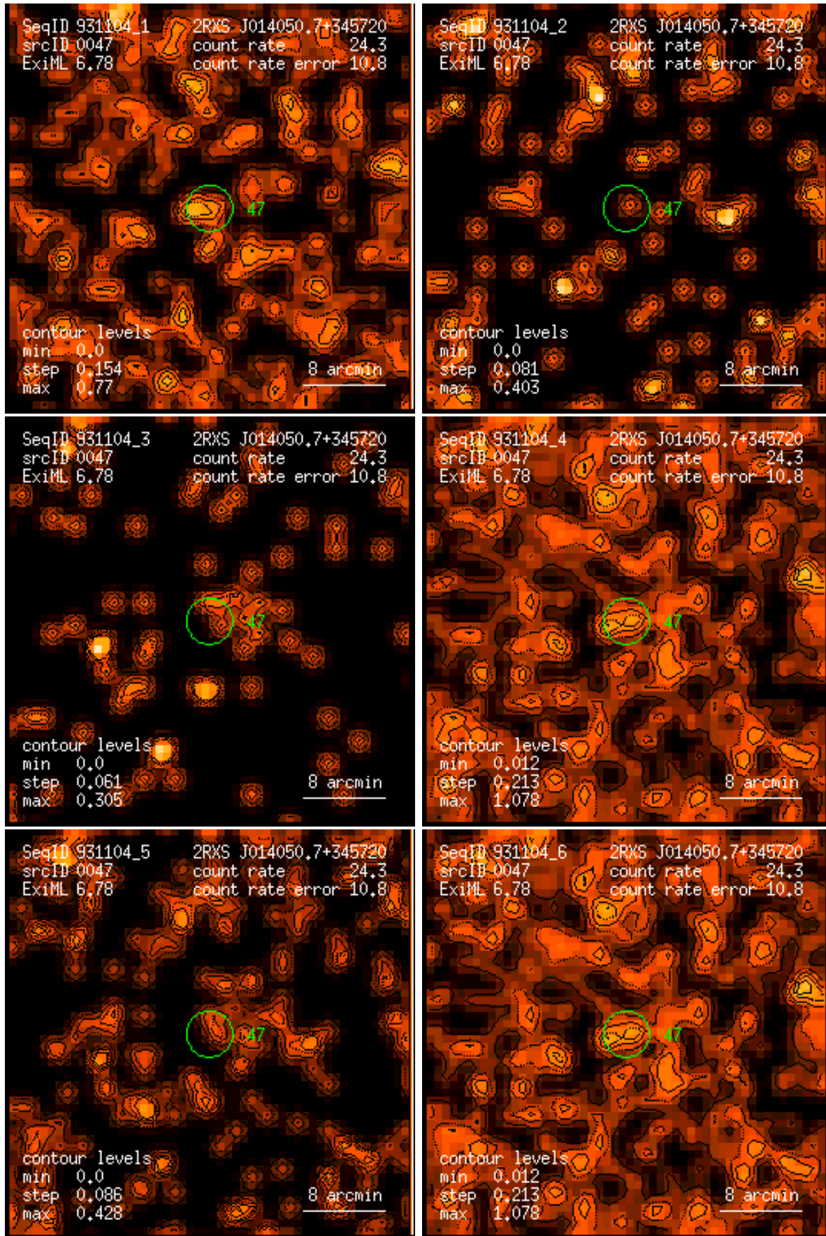
Figure 47: RASS 931104: detection 0047: band rate images, Gaussian filter: (1) PSPC channels 11 – 41, (2) 52 – 90, (3) 91 – 201, (4) 11 – 235, (5) 52 – 201, (6) 11 – 201. Broad band rates in counts/ks. Band rate contour levels in counts/ks/arcmin 2 .
