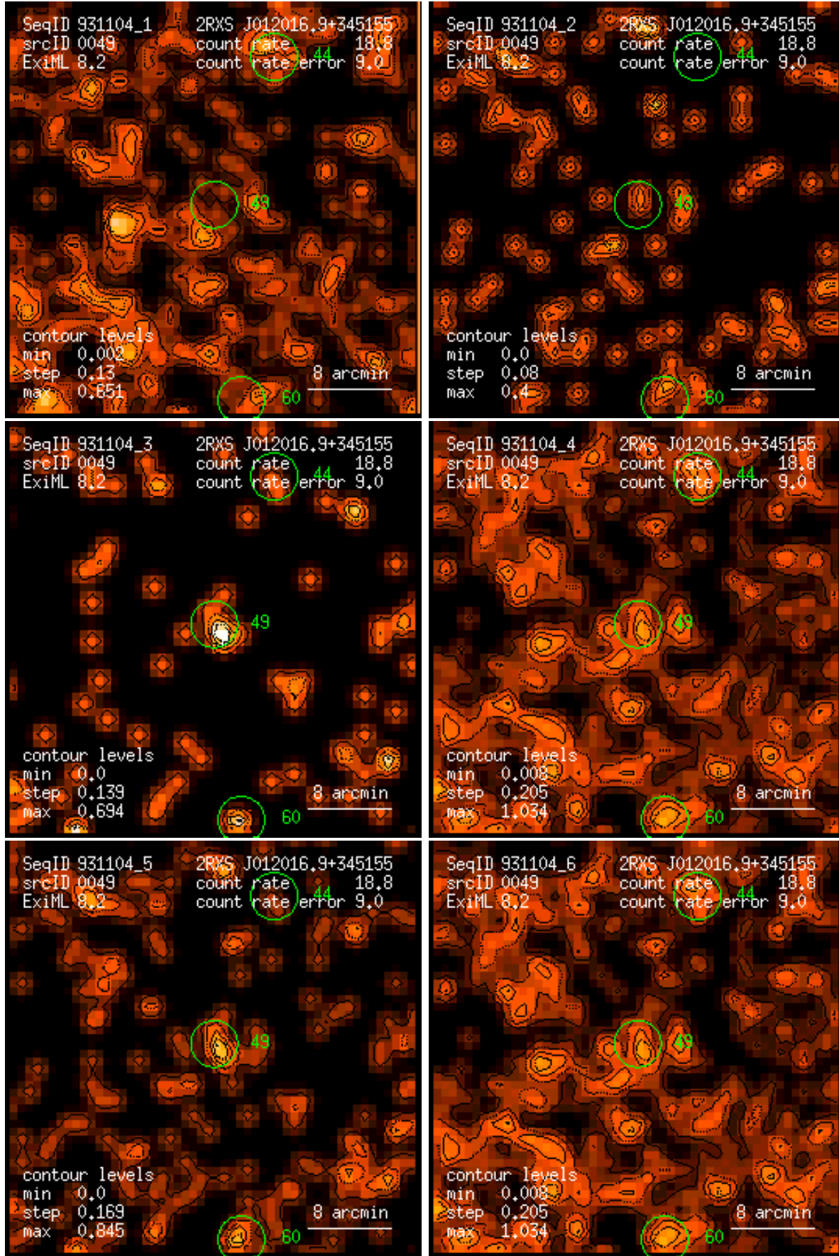
Figure 49: RASS 931104: detection 0049: band rate images, Gaussian filter: (1) PSPC channels 11 – 41, (2) 52 – 90, (3) 91 – 201, (4) 11 – 235, (5) 52 – 201, (6) 11 – 201. Broad band rates in counts/ks. Band rate contour levels in counts/ks/arcmin 2 .
