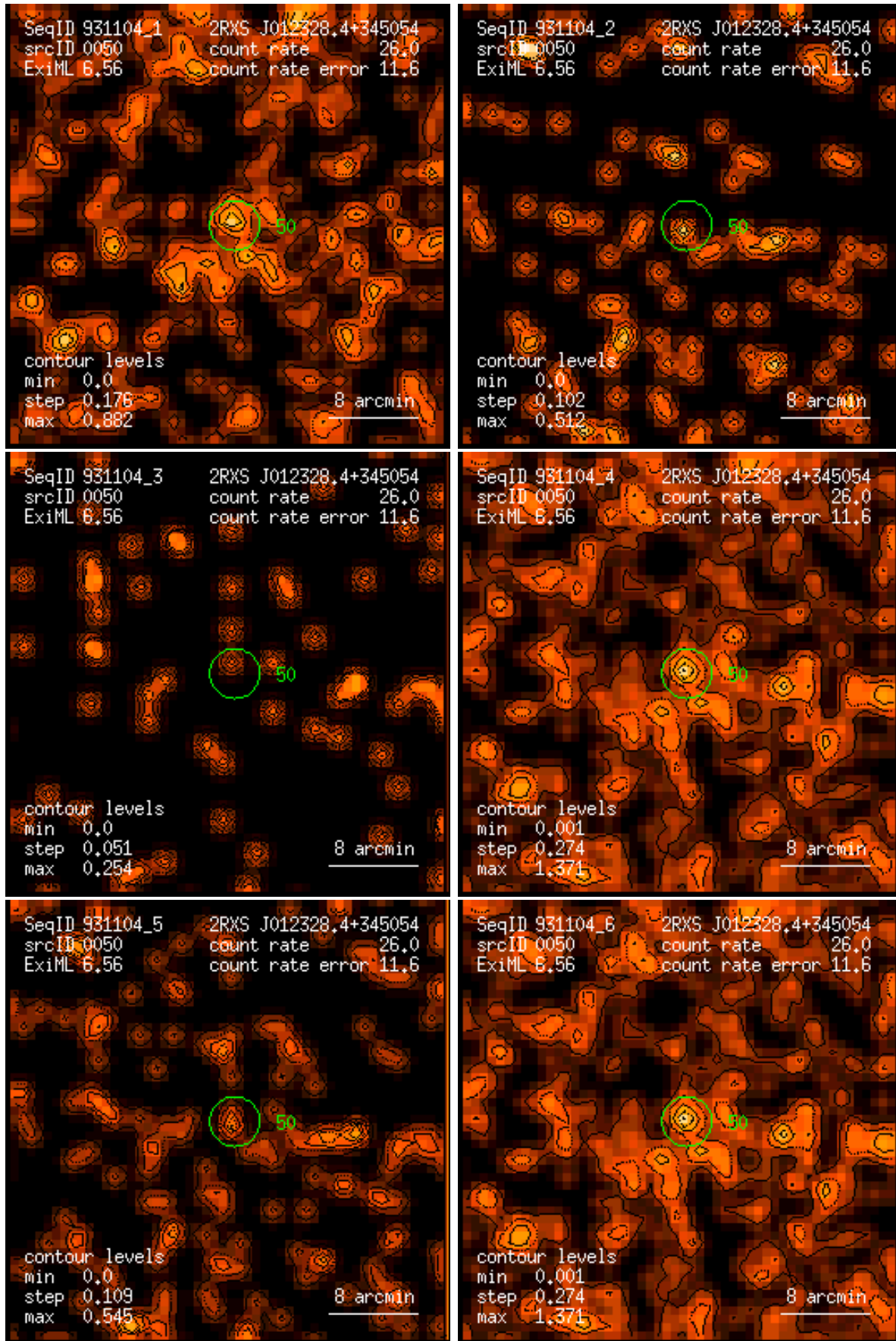
Figure 50: RASS 931104: detection 0050: band rate images, Gaussian filter: (1) PSPC channels 11 – 41, (2) 52 – 90, (3) 91 – 201, (4) 11 – 235, (5) 52 – 201, (6) 11 – 201. Broad band rates in counts/ks. Band rate contour levels in counts/ks/arcmin 2 .
