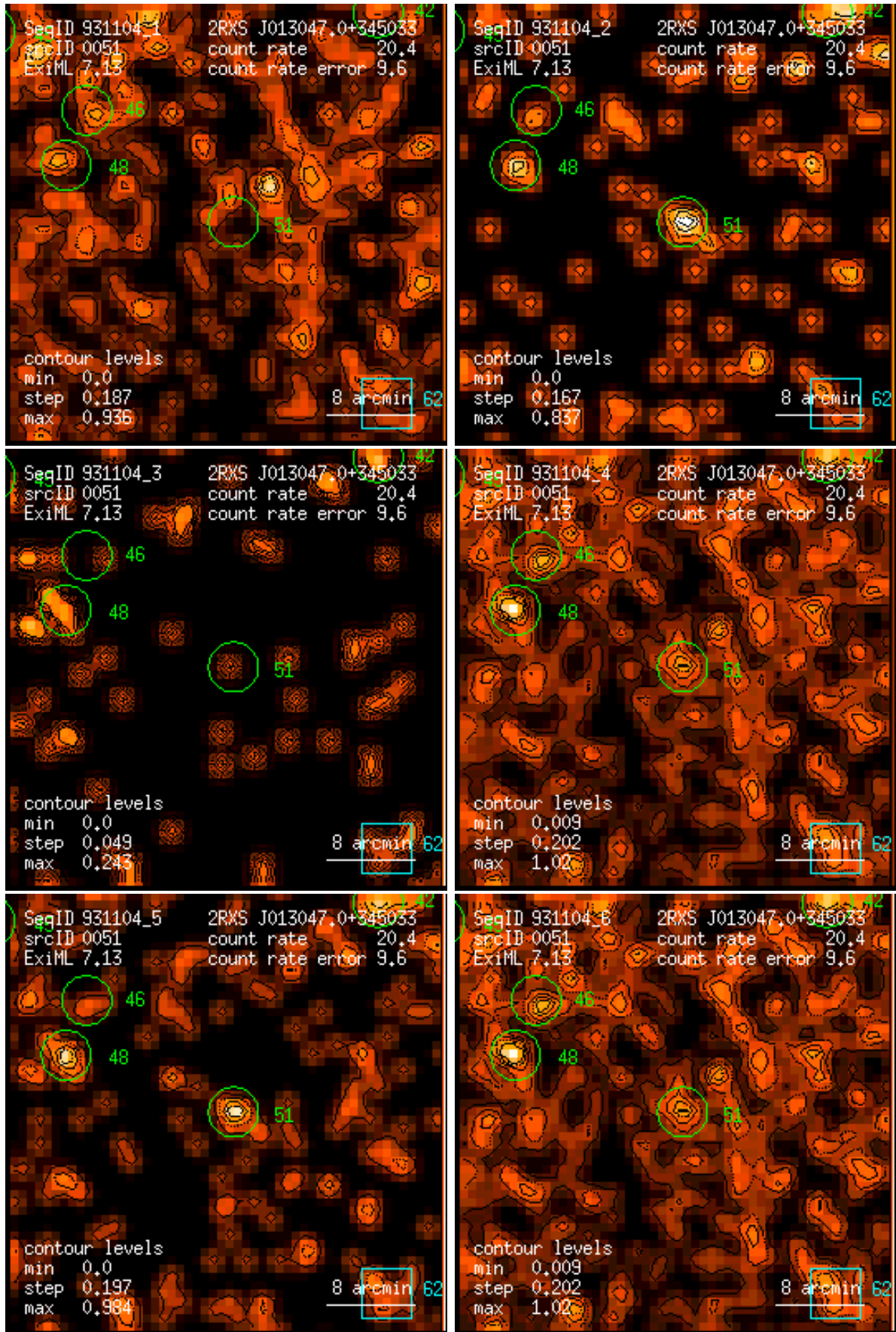
Figure 51: RASS 931104: detection 0051: band rate images, Gaussian filter: (1) PSPC channels 11 – 41, (2) 52 – 90, (3) 91 – 201, (4) 11 – 235, (5) 52 – 201, (6) 11 – 201. Broad band rates in counts/ks. Band rate contour levels in counts/ks/arcmin 2 .
