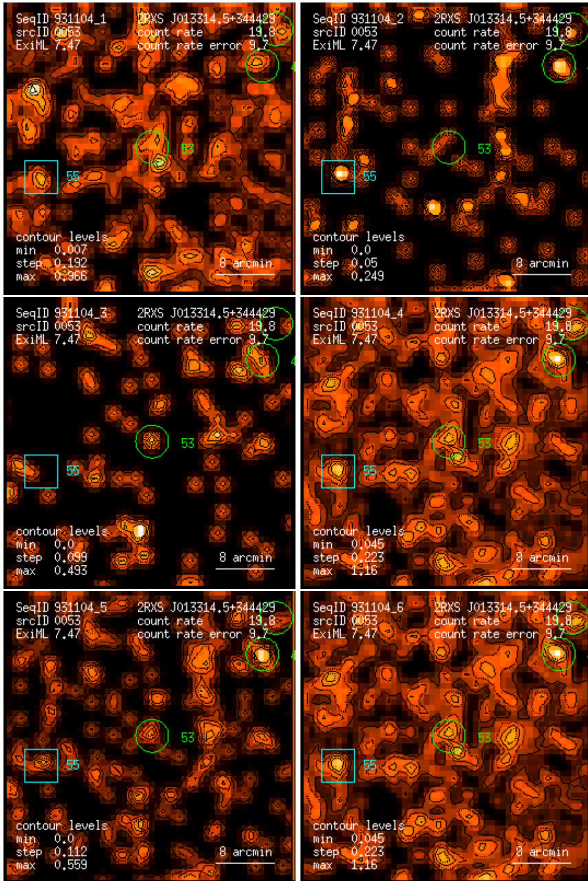
Figure 53: RASS 931104: detection 0053: band rate images, Gaussian filter: (1) PSPC channels 11 – 41, (2) 52 – 90, (3) 91 – 201, (4) 11 – 235, (5) 52 – 201, (6) 11 – 201. Broad band rates in counts/ks. Band rate contour levels in counts/ks/arcmin 2 .
